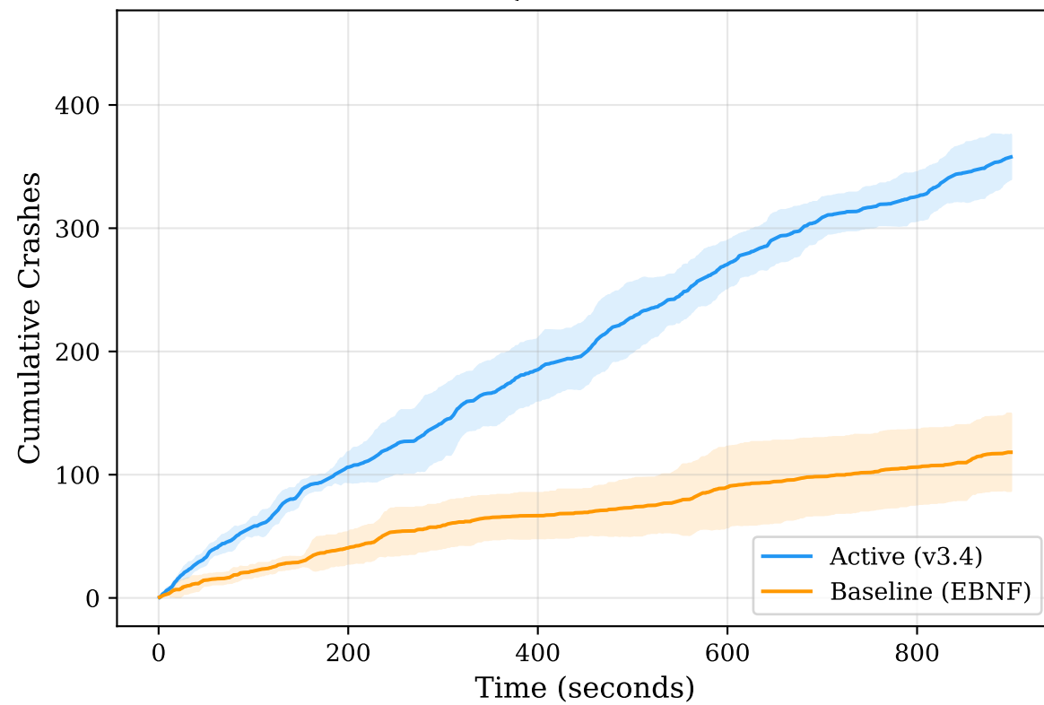
SQLite 3.32.0
