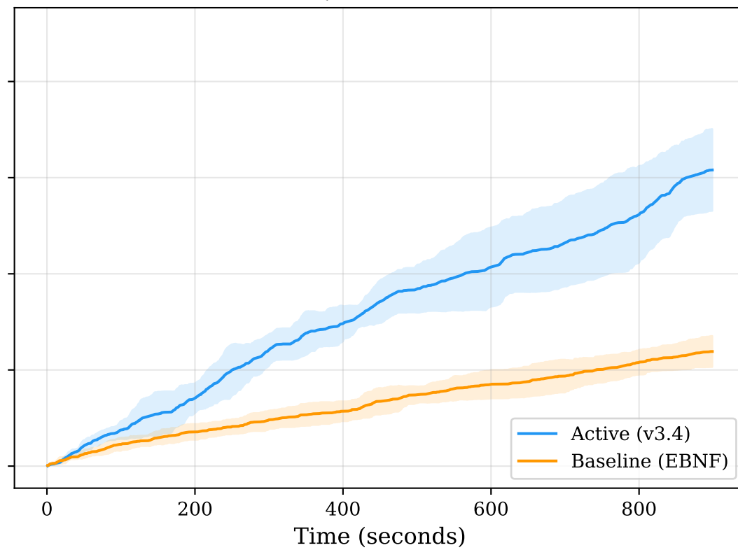
SQLite 3.32.2
