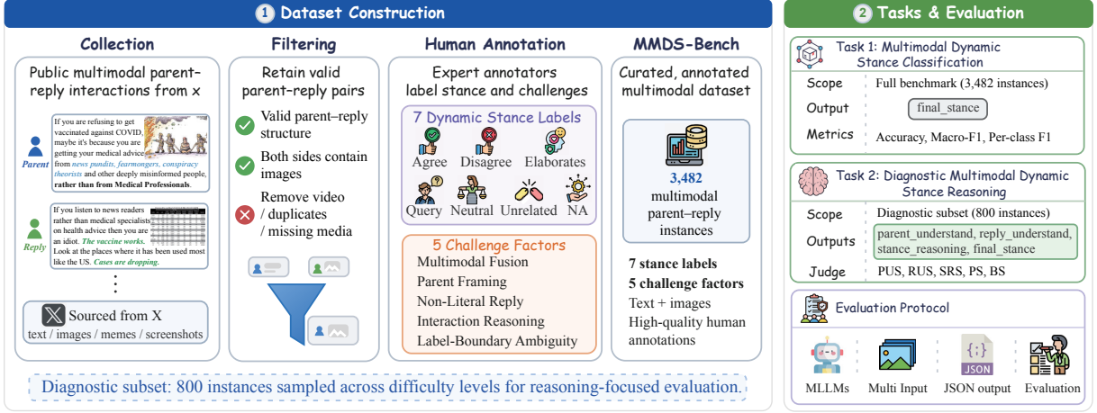
Figure 1: Overview of the dataset construction, tasks, and evaluation in MMDS-Bench.
