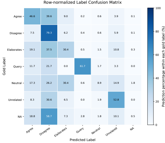
Figure 3: Row-normalized label confusion matrix for Task 1. Rows denote gold labels and columns denote predicted labels. Each cell indicates the percentage of predictions assigned to the corresponding predicted label within each gold-label group.
