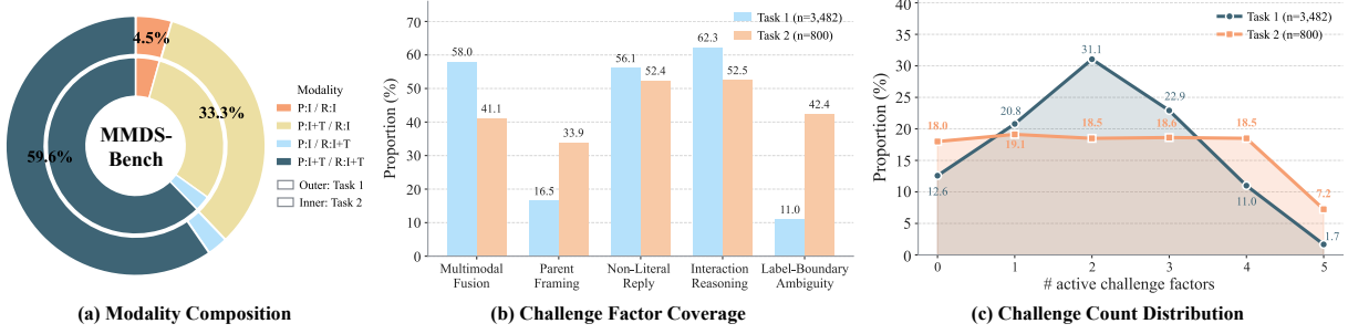
Figure 2: MMDS-Bench dataset statistics. (a) Modality composition (outer ring: Task 1; inner ring: Task 2; P = parent, R = reply, I = image, and T = text), (b) per-instance coverage of the five challenge factors, and (c) distribution of the number of active challenge factors per instance. Task 1 ( n=3,482 ) covers the full benchmark; Task 2 ( n=800 ) is the diagnostic subset, sampled approximately uniformly across challenge-count groups to balance difficulty.
