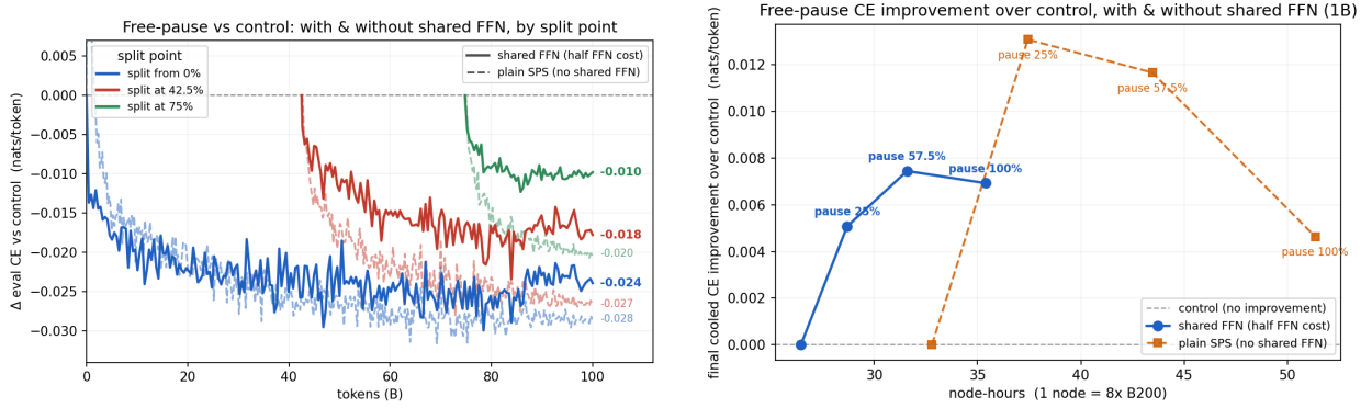
Figure 4: Shared gated FFN vs the two-pass free pause. Left : change in eval CE against control by split point; solid = shared FFN, dashed = two-pass. The shared form keeps most of the advantage at half the FFN cost. Right : final cooled CE improvement over each variant’s own control vs node-hours—this normalizes out the different baselines. The shared-FFN frontier (blue) reaches its gain at far fewer node-hours than the two-pass form (orange).
