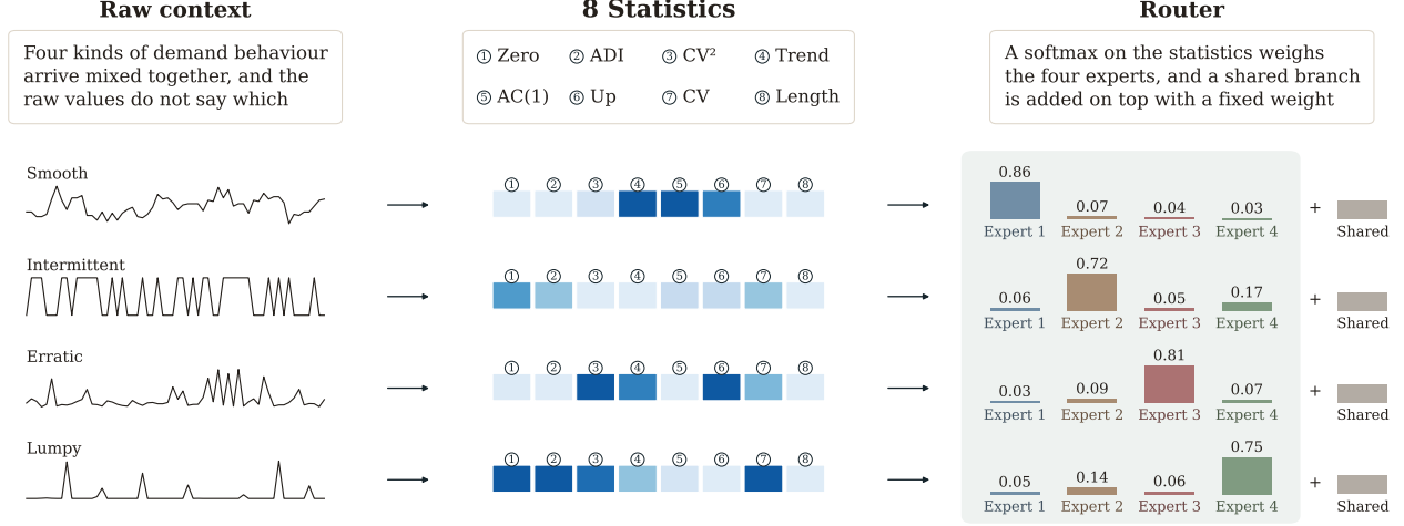
Figure 8: EXAONE Demand on the four demand classes. (1) Raw context : The window that the model receives, with no rescaling of its values. (2) 8 Statistics : The scale-free summary that the window is reduced to. (3) Router : One weight per routed branch, with the always-on shared branch added at a fixed weight.
