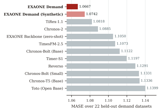
Figure 2: Performance on demand datasets.
