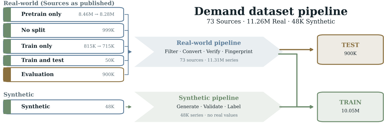
Figure 4: Pipeline for demand dataset construction. 1) Collection: Real sources are grouped by their published role, and the synthetic corpus forms a group of its own below. 2) Preprocessing: The two corpora run on separate tracks. The real track filters, converts, and verifies each source before removing leaked series, while the synthetic track generates, validates, and labels its own. 3) Train-test split: Of the five roles, only the evaluation suites reach the test side, and the other four are used for training, together with every one of the synthetic series.
