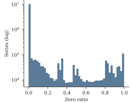
Figure 5: Zeros in the corpus. Zeros are absent from most series, and intermittency is therefore concentrated in a minority.
