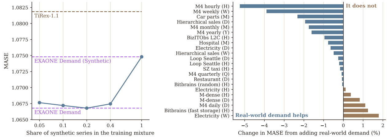
Figure 13: What the training data contributes. [Left] The share of synthetic series in the mixture, where each point is the median of three seeds except the synthetic-only point at 1.0, which is the median of its own runs. [Right] The change in MASE from adding real-world demand to the synthetic corpus, on the 22 datasets in the evaluation suite.
