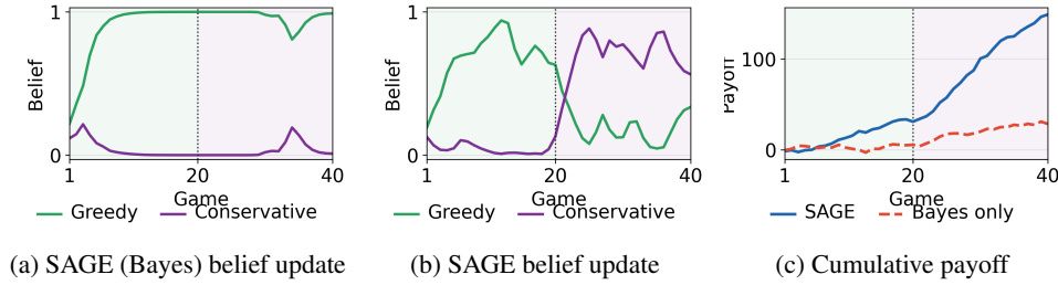
Figure 10: Goofspiel adaptation after a Greedy-to-Conservative opponent shift.
