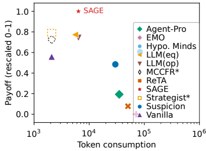
Figure 2: Token consumption-payoff comparison between different methods. * denotes non-LLM agents.
