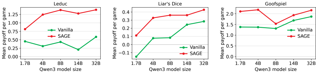
Figure 8: Performance scaling with LLM size.
