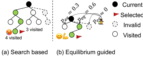
Figure 4: Comparison between search-based lookahead and our method.
