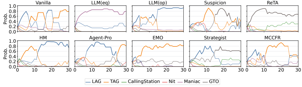
(a) Leduc Hold'em
