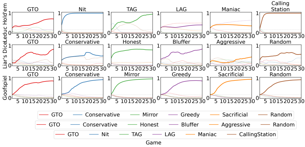
Figure 12: Opponent-belief dynamics across common types of opponents. Each panel shows the belief distribution over opponent styles during 30 games; the thick curve corresponds to the true opponent style, while dashed curves correspond to other styles.
