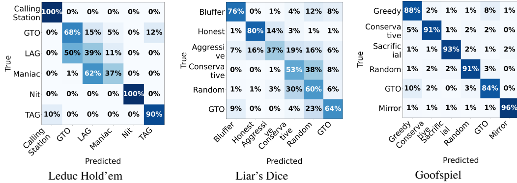
Figure 14: Confusion matrices for the online belief model. Rows correspond to the intended opponent style and columns correspond to the style receiving the largest belief mass.
