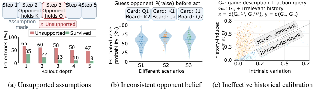
Figure 1: Observed vulnerabilities of free-form LLM strategic reasoning (Leduc Hold'em).
