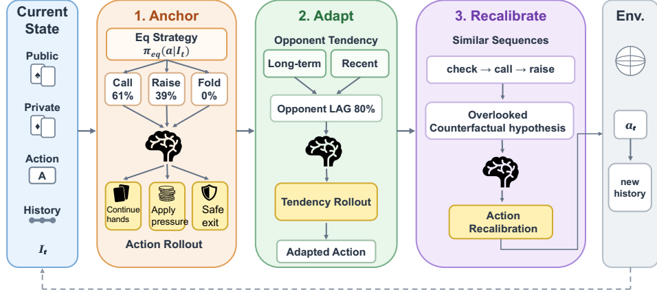
Figure 3: Overview of SAGE. It uses an equilibrium policy as a strategic starting point and opponent estimates as contextual guidance. When matched historical interactions are available, it additionally provides counterfactual hypotheses for the current decision.
