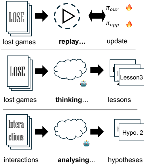
Figure 5: Difference between policy update methods, lesson methods and ours.
