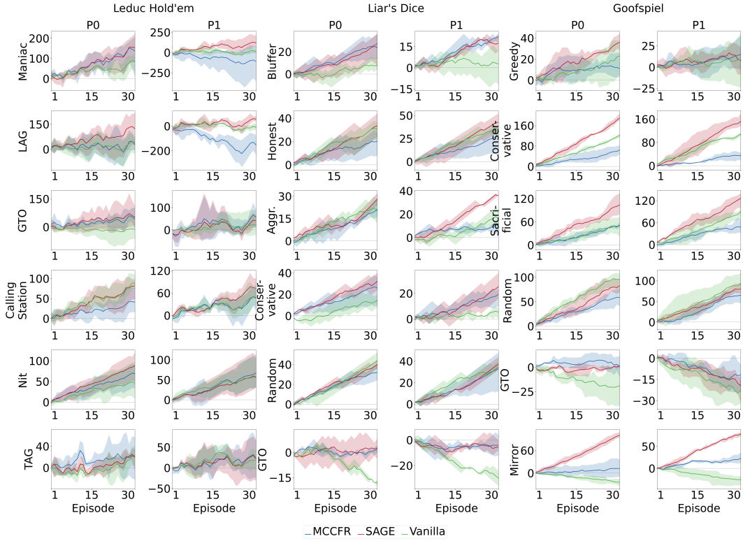
Figure 11: Payoff dynamics over repeated interaction. Each panel compares SAGE with the MCCFR policy baseline and the vanilla LLM baseline, reporting mean cumulative payoff over 30 episodes for one game, opponent style, and player position. Curves are averaged across 5 runs, and shaded regions indicate cross-run variability.
