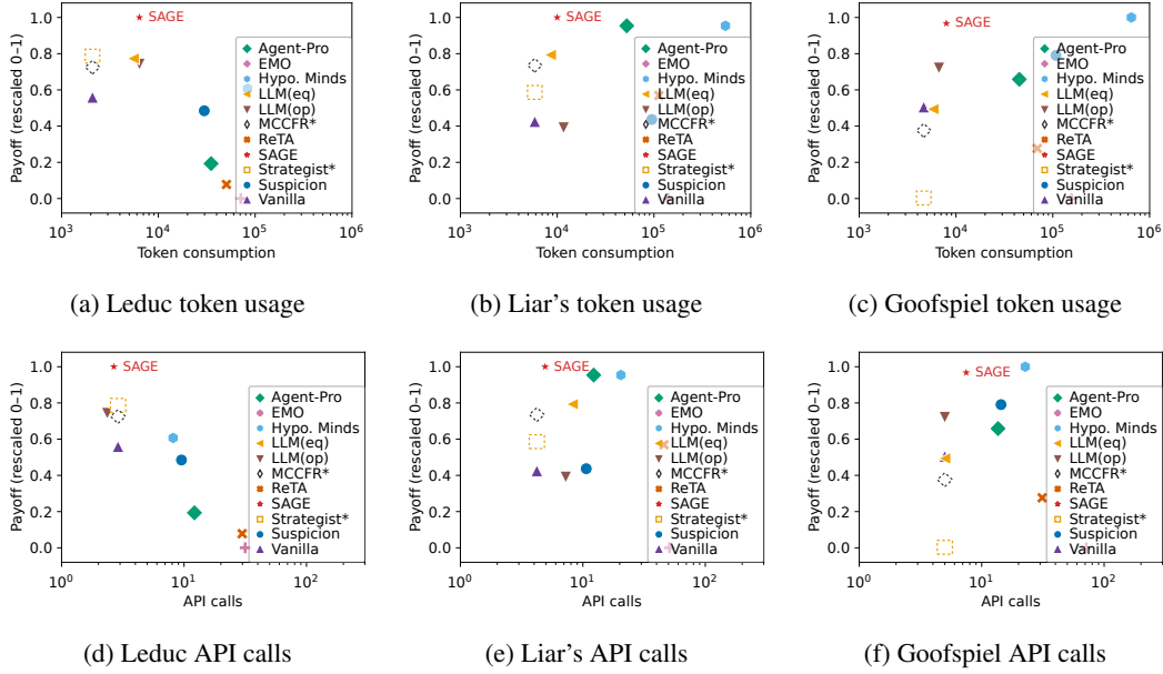
Figure 6: Performance–efficiency comparison across three games. The top row reports token consumption and the bottom row reports API calls. Payoff is min–max rescaled across methods within each game; both efficiency axes use a log scale. MCCFR* and Strategist* do not involve LLM inference and are shown as blank icons for payoff comparison.
