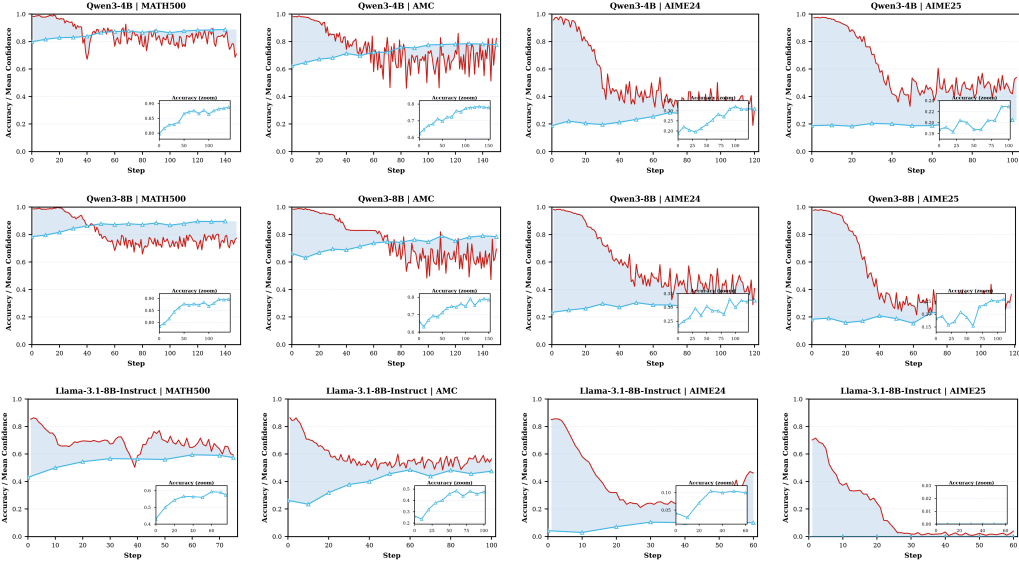
Figure 11: More training dynamics of TTCL on base models. The red curves show mean confidence and the cyan-blue curves show empirical accuracy during TTCL training. The shaded area indicates the confidence-accuracy gap, and the inset zooms in on the accuracy trajectory. TTCL progressively aligns confidence with empirical accuracy while improving task accuracy.
