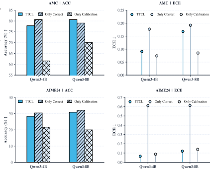
Figure 4: Ablation study. “Only Correct” and “Only Calibration” retain correctness and calibration rewards, respectively.
