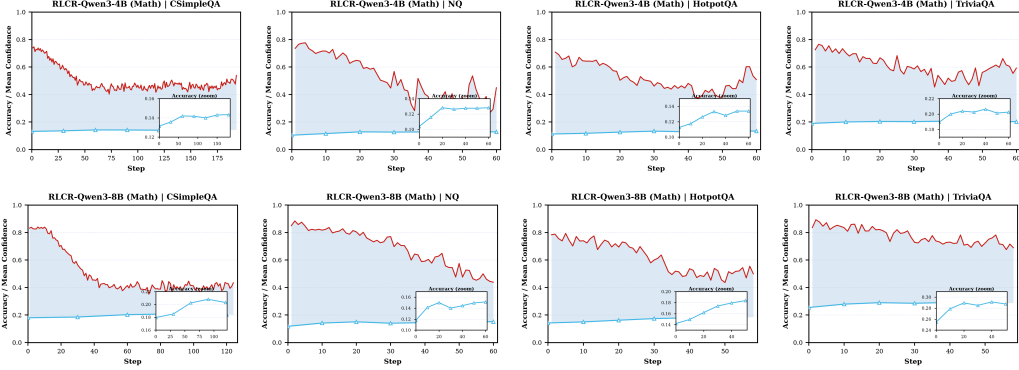
Figure 12: More training dynamics of TTCL on calibrated models. The red curves show mean confidence and the cyan-blue curves show empirical accuracy during TTCL training. The shaded area indicates the confidence-accuracy gap, and the inset zooms in on the accuracy trajectory. TTCL progressively aligns confidence with empirical accuracy while improving task accuracy.
