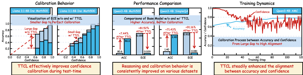
Figure 1: Overview of our work: TTCL enables label-free calibration learning directly on unlabeled target-task data, consistently improving reasoning accuracy while reducing calibration error across models and tasks, with confidence progressively aligning with accuracy during test-time learning.
