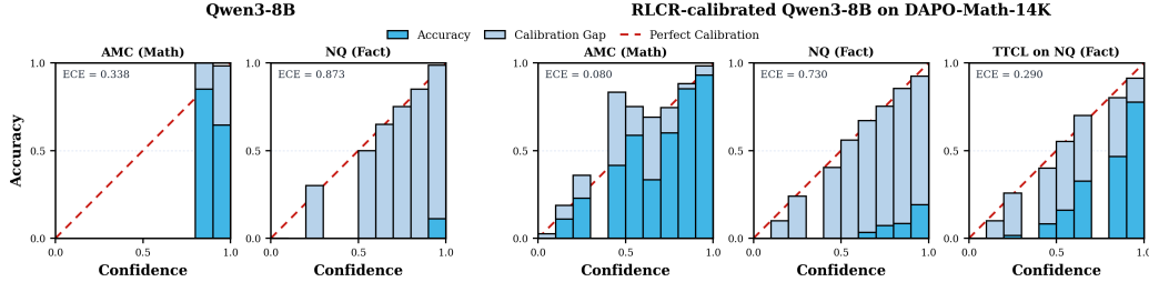
Figure 2: Calibration performance of Qwen3-8B and its RLCR-calibrated model on DAPO-Math-14K. Left: Base Qwen3-8B exhibits over-confidence on both AMC and NQ, with predicted confidence exceeding empirical accuracy. Right: RLCR on DAPO-Math-14K transfers well to AMC but remains limited on NQ, where further TTCL adaptation markedly improves calibration.
