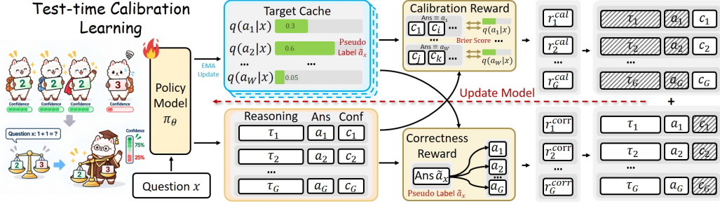
Figure 3: Illustration of TTCL method: Given an unlabeled question, TTCL samples multiple rollouts to construct label-free supervision: the most supported answer serves as the pseudo label, while the support of each answer provides its confidence target. A target cache stabilizes these signals and is updated via EMA across epochs. Correctness and calibration rewards are optimized separately, with the former updating reasoning and answer tokens and the latter updating only confidence tokens.
