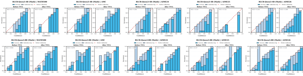
Figure 9: Visualization of in-domain calibration effects before and after TTCL on math-calibrated models for mathematical benchmarks. TTCL calibrates models to the target benchmarks, further narrowing the gap between confidence and empirical accuracy. Blue bars denote empirical accuracy within each confidence bin, while light blue bars indicate the deviation from perfect calibration.
