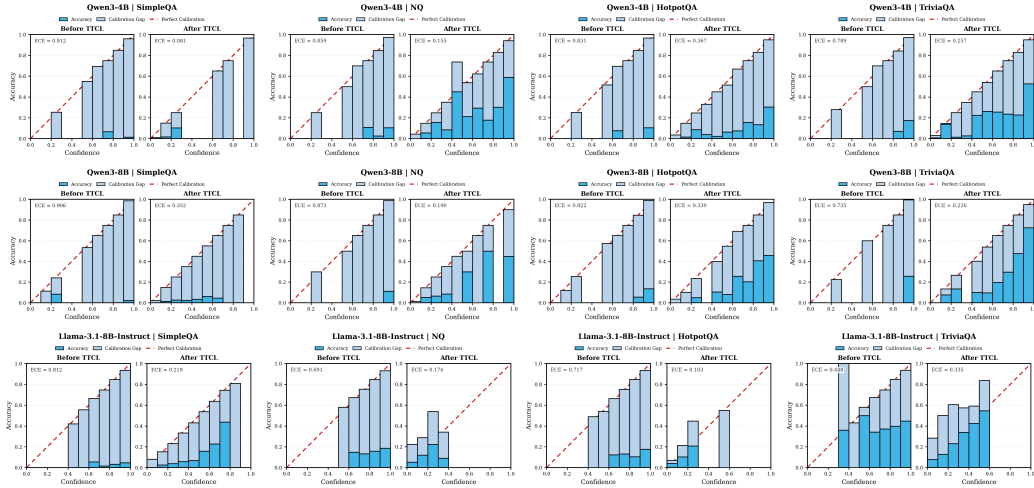
Figure 8: Visualization of calibration effects before and after TTCL on base models for factual QA benchmarks. TTCL effectively calibrates models to the target benchmarks, substantially narrowing the gap between confidence and empirical accuracy. Blue bars denote empirical accuracy within each confidence bin, while light blue bars indicate the deviation from perfect calibration.
