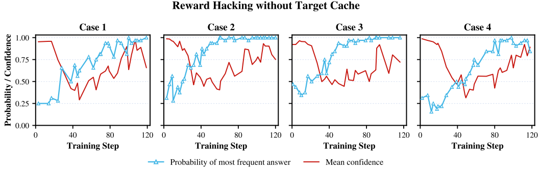
Figure 13: Reward hacking without the target cache. Four AIME24 examples in which the model’s rollouts increasingly concentrate on an incorrect answer while mean confidence rises toward 1.0. The blue lines show the frequency-based probability of the most frequent answer, and the red lines show mean confidence. When supervision signals are derived from the the rollout group of current policy, increasing agreement on a wrong answer raises its confidence target, leading to reward hacking.
