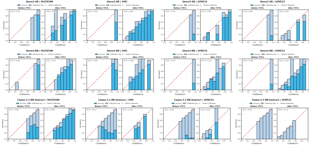
Figure 7: Visualization of calibration effects before and after TTCL on base models for mathematical benchmarks. TTCL effectively calibrates models to the target benchmarks, substantially narrowing the gap between confidence and empirical accuracy. Blue bars denote empirical accuracy within each confidence bin, while light blue bars indicate the deviation from perfect calibration. For Llama-3.1-8B-Instruct on AIME25, no accuracy bars is shown because its empirical accuracy is 0.
