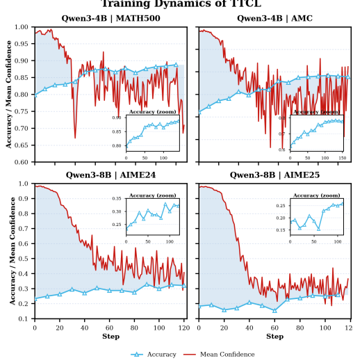
Figure 5: Training dynamics of TTCL. The dynamics illustrate the calibration process between accuracy and mean confidence during TTCL training. More dynamics refer to Appendix F.3.
