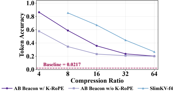
Figure 6: Reconstruction accuracy from compressed beacon states on length-16,384 random sequences over 46 symbols, averaged over three seeds. SlimKV starts from 8\times total compression due to 4\times feature compression. Dashed line denotes random-guessing probability.
