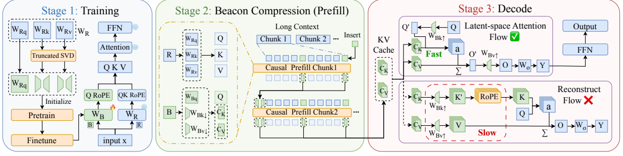
Figure 3: Overview of SlimKV. SlimKV trains low-rank beacon KV projections and caches only latent beacon KV states after prefill. During decoding, SlimKV performs latent-space attention over cached beacon memories, avoiding full-dimensional reconstruction.
