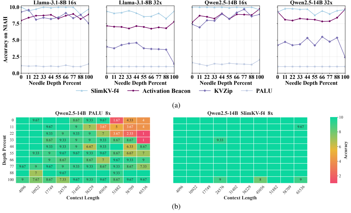
Figure 7: Needle-in-a-Haystack evaluation. (a) SlimKV outperforms baselines across depths under 16\times and 32\times compression. (b) SlimKV maintains retrieval ability for information beyond Qwen2.5-14B’s context window (32K). Since higher ratios limit PALU’s retrieval accuracy, we select 8\times compression to better reveal the behavior.
