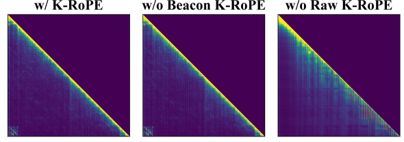
Figure 5: Attention maps under K-RoPE ablations. Beacon K-RoPE removal remains much closer to the K-RoPE-kept pattern than raw-token K-RoPE removal.
