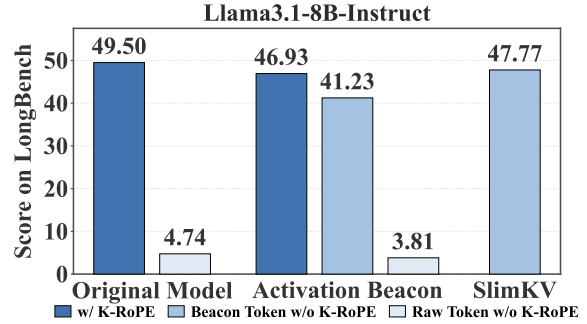
Figure 2: LongBench scores under K-RoPE ablations, showing positional asymmetry between raw and beacon tokens. SlimKV remains close to the original model without beacon K-RoPE.
