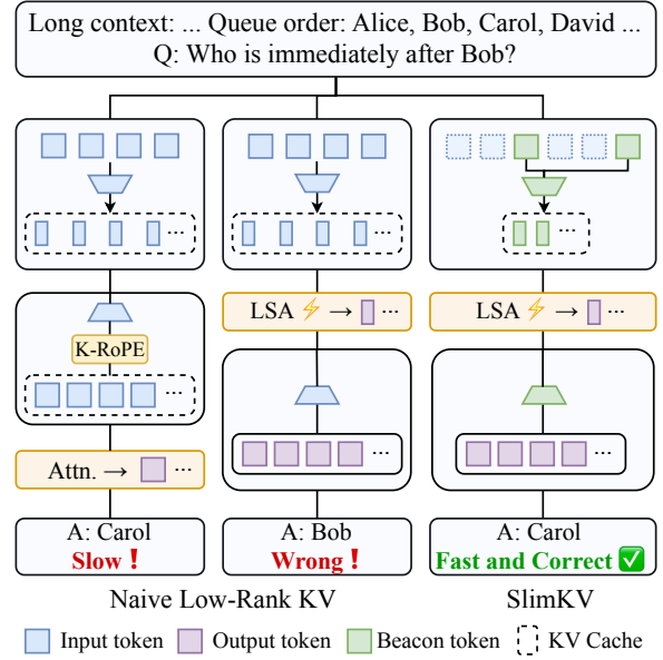
Figure 1: Comparison of low-rank KV-cache strategies. K-RoPE forces reconstruction, while its removal enables latent-space attention (LSA) but loses order information. SlimKV uses K-RoPE-free beacon tokens to retain semantics and positional cues in latent KV space.
