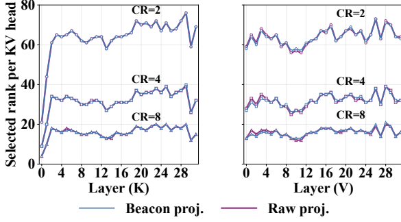
Figure 4: Layer-wise rank allocation. K/V ranks of Beacon and raw weights in Llama-3.1-8B under 2\times , 4\times , and 8\times feature compression, selected by equal explained variance.
