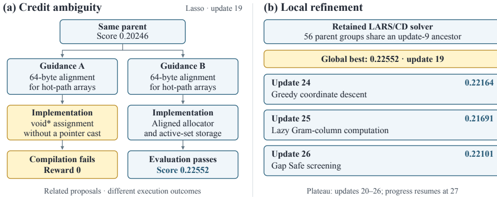
Figure 12: Lasso examples of the same two failure structures studied in Polyomino and TriMul. (a) Related alignment proposals from one parent have different outcomes because one implementation contains a pointer-conversion error. (b) During a seven-update plateau, all selected parents share an update-9 ancestor; the displayed step-best programs refine the retained LARS/CD solver without exceeding the update-19 frontier. Values are search-time scores, not fixed-program re-evaluation means.
