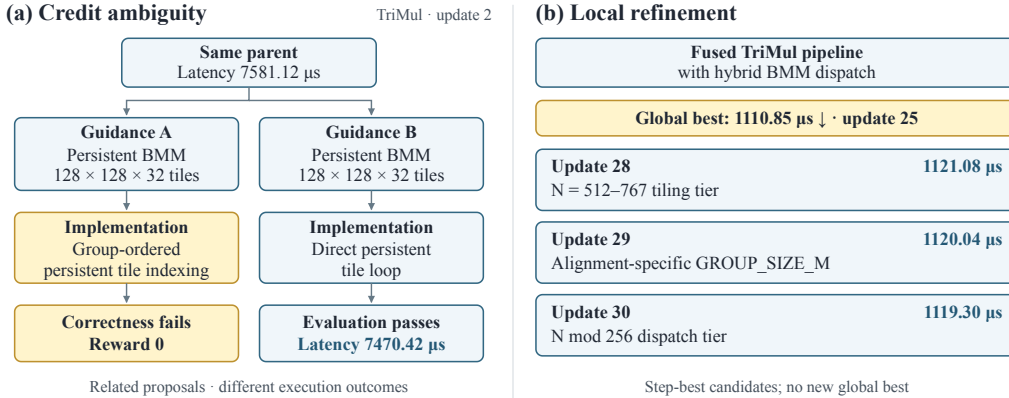
Figure 11: TriMul cases corresponding to the two failure modes in Figure 9. (a) Two proposals from the same parent use the same large- N persistent-BMM schedule, but only one realization passes correctness tests. (b) After the global frontier stops improving at update 25, the step-best candidates at updates 28–30 continue to refine BMM tiling and dispatch within the same kernel family.
