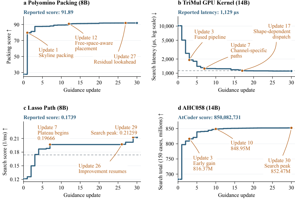
Figure 6: Best-so-far search trajectories under GLM-5.2 execution. Search scores and Table 2 results use different evaluation environments.
