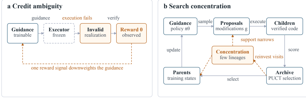
Figure 9: Two failure modes in Guidance-TTT. (a) Execution failures can assign zero reward to useful guidance. (b) The archive–policy loop can concentrate training and search within a few successful lineages.
