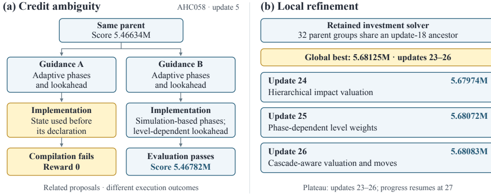
Figure 13: AHC058 counterparts of the Polyomino/TriMul failure cases. (a) Related proposals request adaptive investment phases and lookahead; one execution fails on a declaration-order error while another passes the judge. (b) During updates 23–26, selected parents share an update-18 ancestor and useful local changes do not improve the frontier. Displayed scores are means over 150 public instances, in millions, rather than the totals used in the main results. Both panels use the 14B-guidance run.
