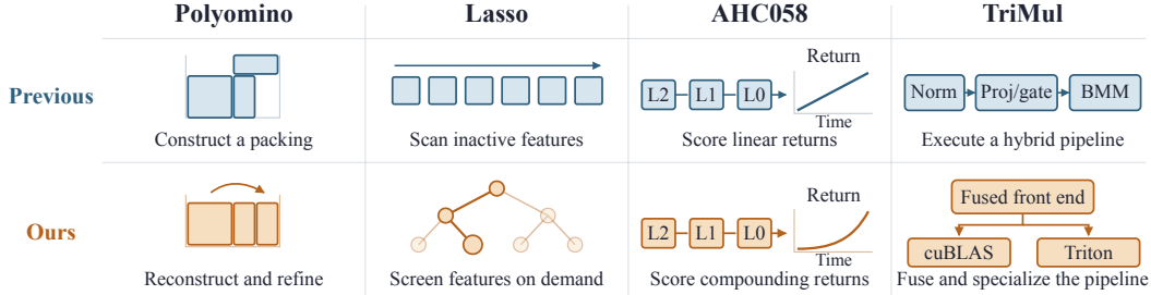
Figure 4: Comparison of solution structures. Blue denotes prior approaches; gold denotes ours.
