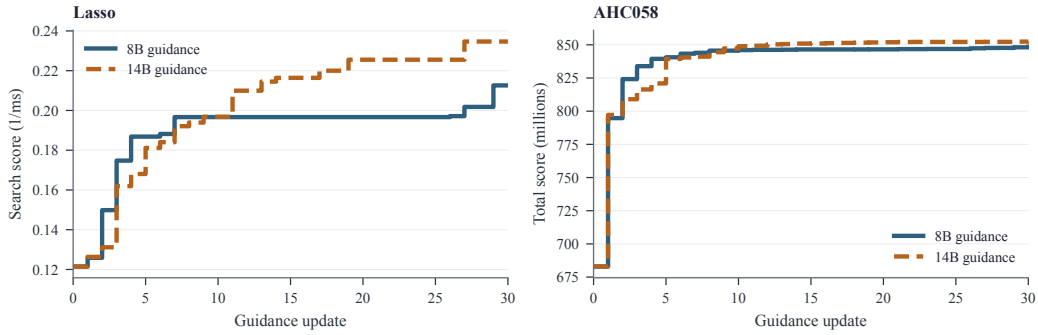
Figure 8: Both guidance sizes on Lasso and AHC058, with the same GLM-5.2 seed within each task. These are search-time archive scores. Lasso’s 14B archive peak (0.23467) exceeds the 8B peak (0.21259), but its frozen-solver mean (0.1730) does not exceed the 8B mean (0.1739).
