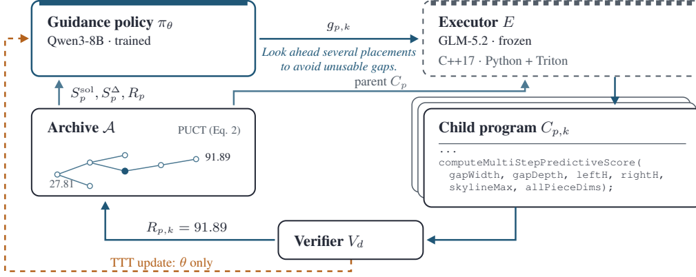
Figure 3: Guidance-TTT workflow. A PUCT-based archive search selects a promising parent solution, the guidance model proposes a high-level modification, and the frozen executor realizes it as a new candidate. The resulting verifier reward updates only the guidance model.
