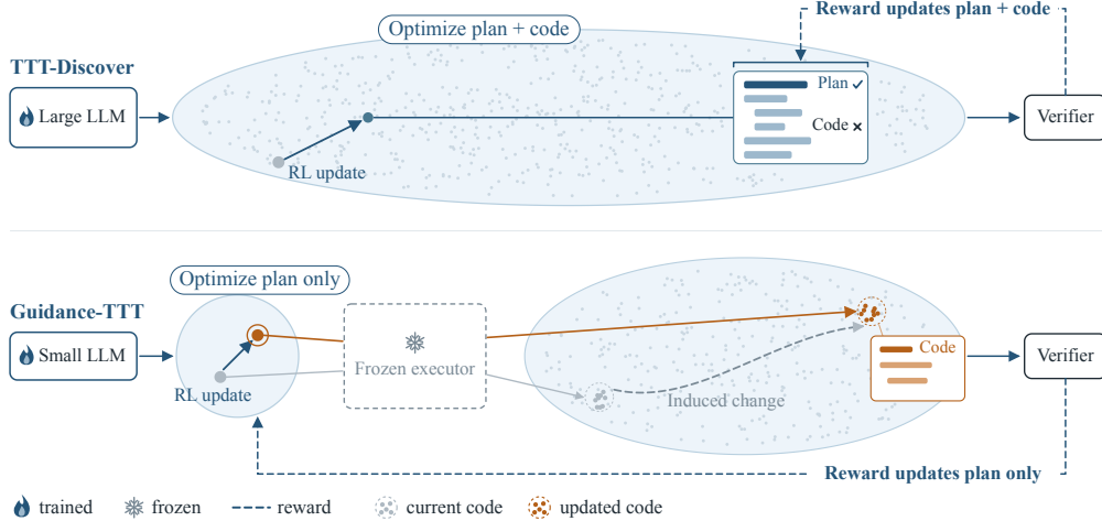
Figure 1: Test-time learning in plan space. TTT-Discover uses verifier reward to update both plan and code generation. Guidance-TTT applies the reward only to the small guidance model, while a frozen executor translates plan changes into code changes.
