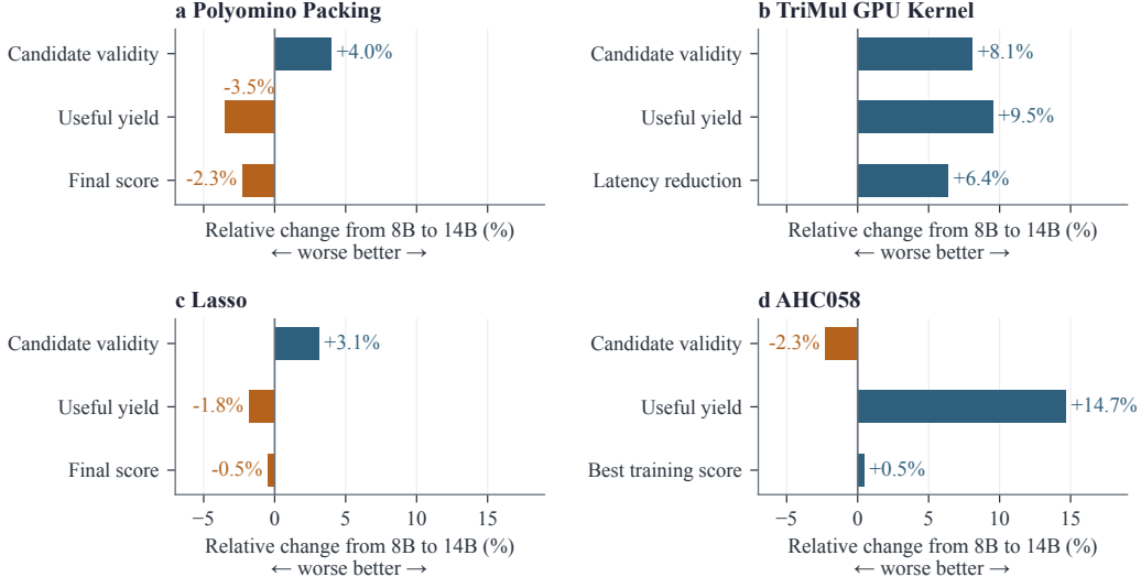
Figure 7: Relative change from 8B to 14B guidance with GLM-5.2 execution. Positive values indicate improvement; TriMul shows relative latency reduction, and AHC058 compares best training-archive scores. TriMul’s 6.4% reduction uses the same-batch means of 1297.44 \mu\text{s} (8B) and 1214.62 \mu\text{s} (14B). Each size has one search trajectory. Raw validity includes service failures, which are audited separately below. Absolute statistics are in Appendix B.1.1.
