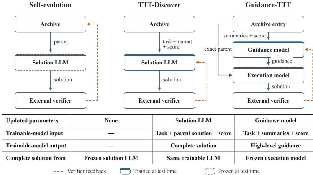
Figure 2: Discovery paradigms differ in where verifier feedback drives adaptation: search in self-evolution, trainable paradigm generation in TTT-Discover, and trainable strategic guidance in Guidance-TTT. Training only the compact guidance model reduces adaptation cost while retaining the implementation capabilities of a stronger, frozen executor.
