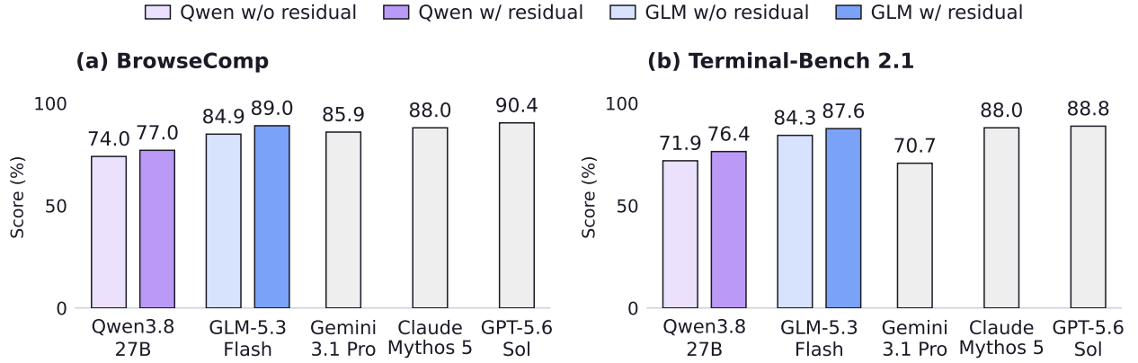
Figure 1: BrowseComp and Terminal-Bench 2.1 scores. Pale and solid bars compare the same local actor without and with residual memory. Gray bars are published frontier references, with their original harnesses and protocols (Google DeepMind, 2026; Terminal-Bench Team, 2026; OpenAI, 2026b); they are not controlled comparisons with our runs.
