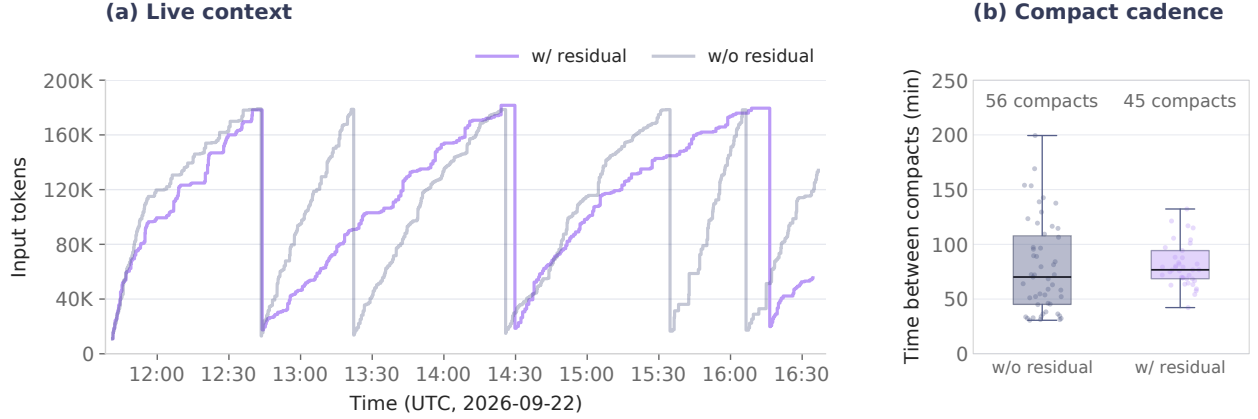
Figure 4: Live Trading context use. (a) An illustrative September 22 trace. (b) Compaction intervals in the separate September 20–23 evaluation: 56/45 completed compactations and 51/41 within-session intervals without/with residual memory. Intervals do not cross restarts; two residual intervals exceed the display range but remain in the box statistics.
