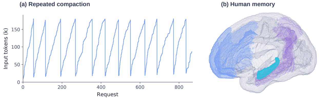
Figure 2: Context compaction and human memory. (a) Input length across successive requests in an agent run, showing repeated growth and sharp reductions. (b) Memory systems illustrated using the Harvard–Oxford atlas (Harvard–Oxford Atlas Contributors, 2026): prefrontal regions (blue), hippocampus (cyan), and association cortex (purple).
