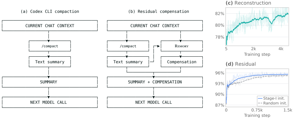
Figure 3: Residual compensation and training. (a) Codex CLI passes the /compact summary to the next actor call. (b) The REMORY network uses that summary to condition memory construction from the active context; summary and continuous memory jointly support subsequent actions. Archive access remains an ordinary tool action in either setting. (c,d) Qwen3.8-27B teacher–student top-1 agreement during Stage I reconstruction and Stage II residual training. The residual panel compares reconstruction initialization with random initialization under the same residual objective and data order. Curves are optimization diagnostics from the training streams.
