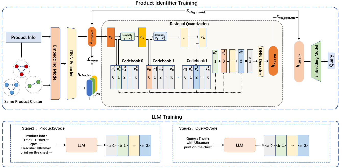
Figure 1: Architecture of our model, consisting of Product Identifier Training and LLM Training.
