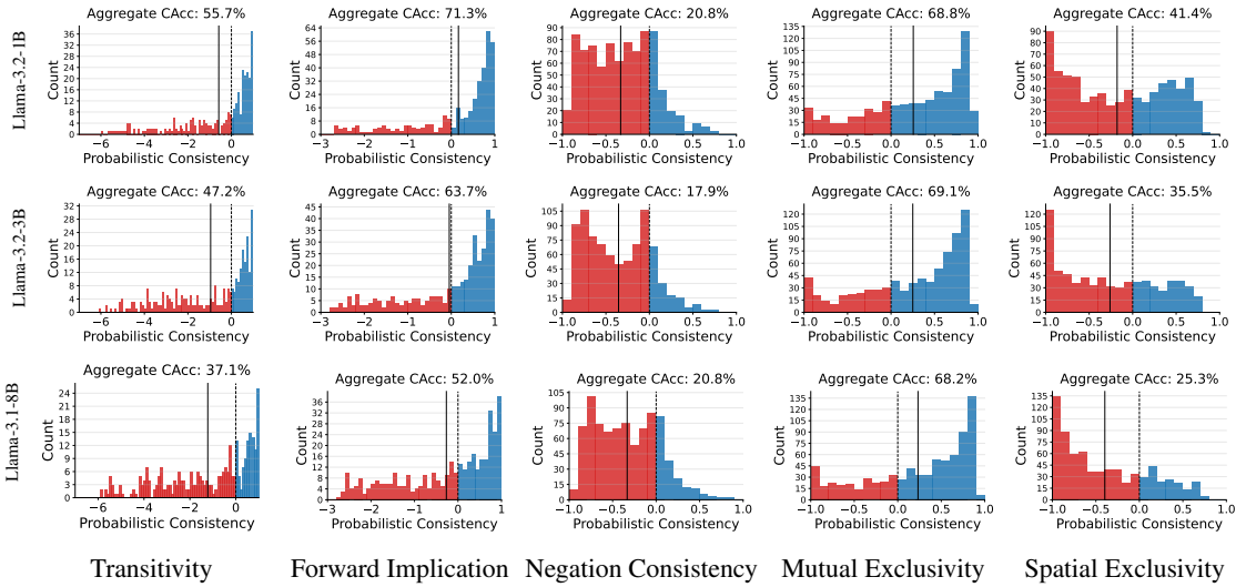
Figure 5: Probabilistic Consistency score distributions for Llama-3 pretrained models using nucleus entropy calibration with nucleus value p = 0.95 . Points highlighted in red are inconsistent, while points highlighted in blue are consistent. The solid vertical black line corresponds to the average probabilistic consistency. Each figure is labeled with the corresponding aggregate CAcc score.
