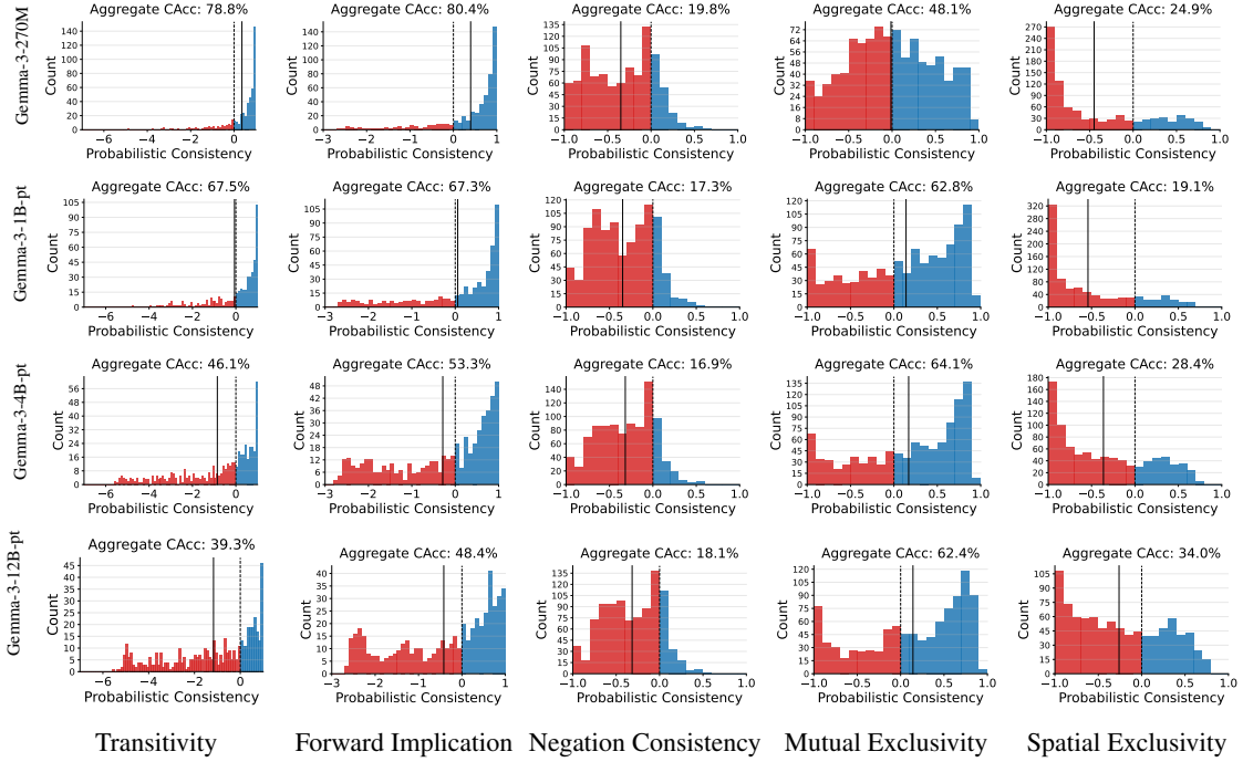
Figure 4: WMC score distributions for Gemma-3 base models using nucleus entropy calibration with nucleus value p = 0.95 . Points highlighted in red are inconsistent, while points highlighted in blue are consistent. The solid vertical black line corresponds to the average probabilistic consistency. Each figure is labeled with the corresponding aggregate CAcc score.
