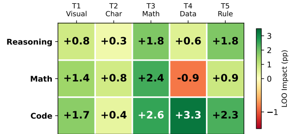
Figure 10: LOO Impact on category averages (Reasoning, Math, Code). Positive values (green) indicate beneficial contribution; negative values (red) indicate interference when included.
