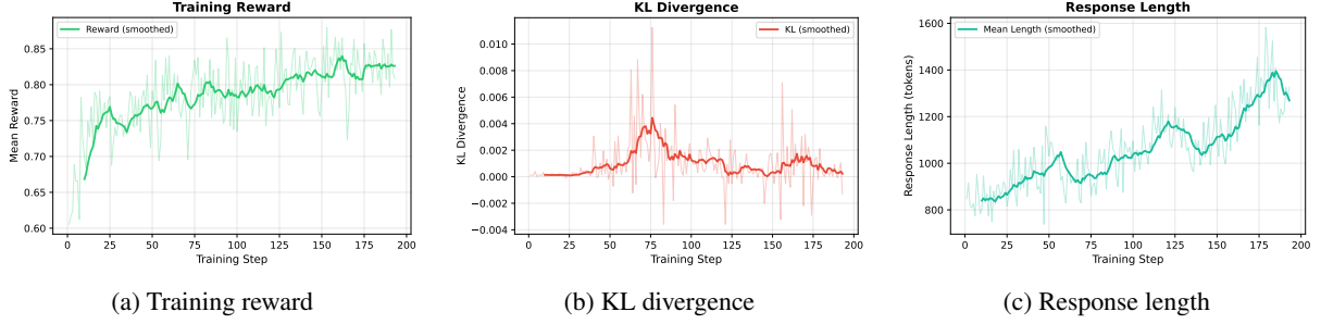
Figure 6: GRPO training dynamics for Qwen3-8B on \mathcal{D}_{\text{mixed}} . (a) Mean reward increases steadily from 0.61 to 0.81, indicating consistent learning. (b) KL divergence remains bounded below 0.004 (smoothed), confirming stable policy updates without reward hacking. (c) Mean response length grows from \sim 850 to \sim 1,330 tokens, reflecting the emergence of more thorough reasoning chains.
