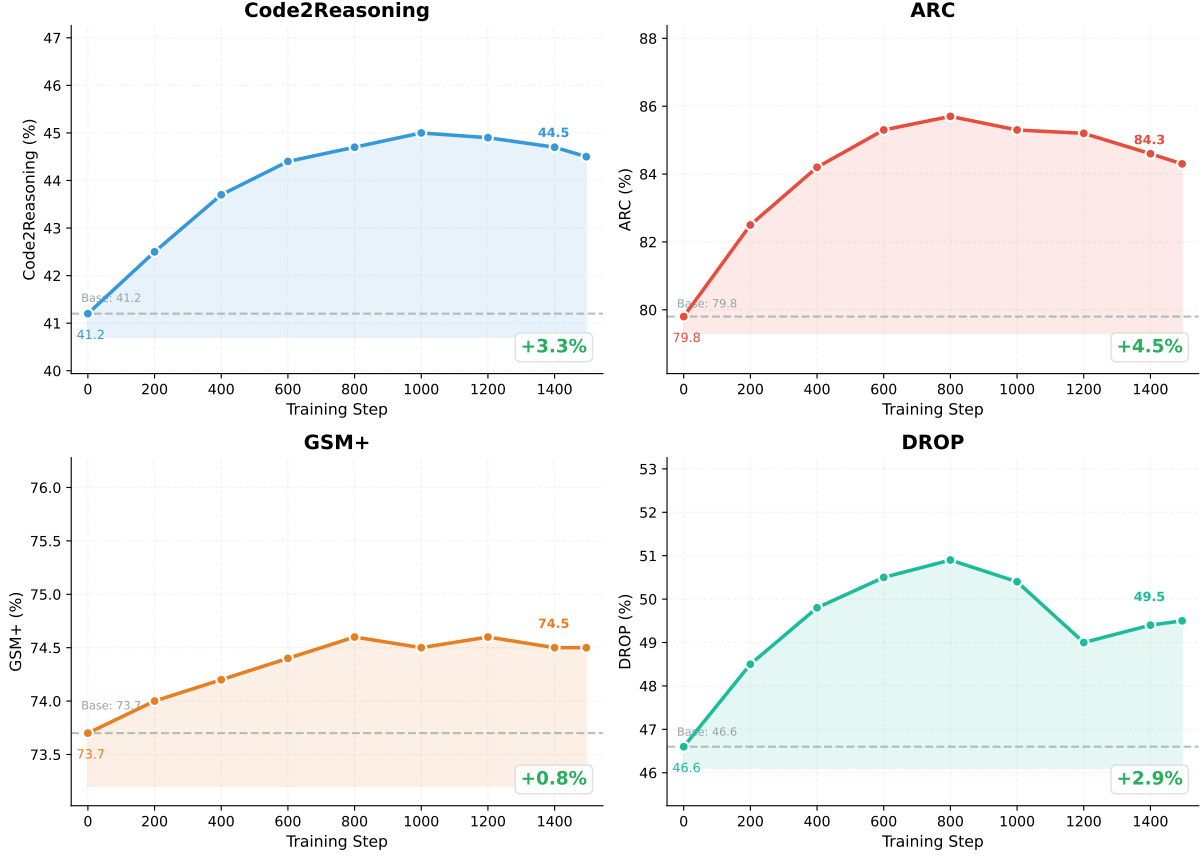
Figure 9: Benchmark evolution during SFT (Qwen3-8B, D_{\text{mixed}} ). Downstream benchmarks show quick initial gains that plateau or slightly decline after step 800, contrasting sharply with the continuous improvement observed under GRPO (Figure 7).
