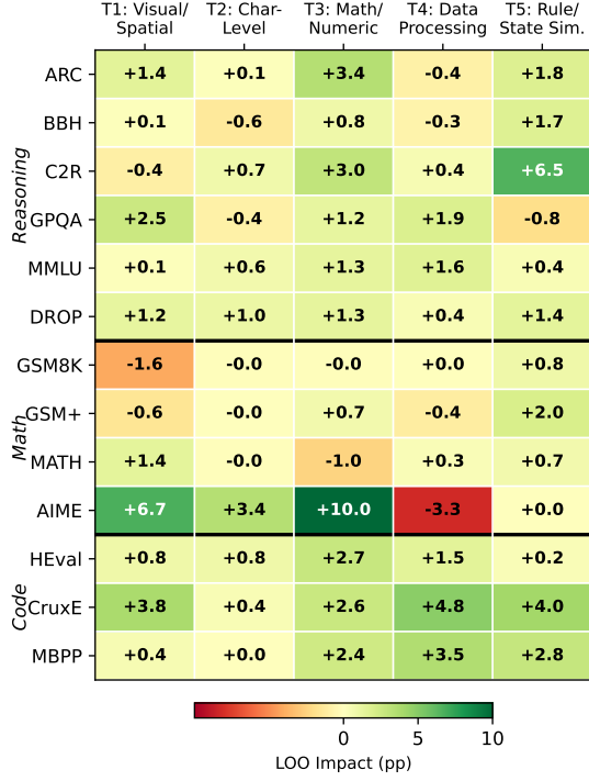
Figure 11: Per-benchmark LOO Impact. Each cell shows the accuracy drop (in percentage points) when the corresponding task type is removed from training. Horizontal lines separate the three evaluation categories: Reasoning, Math, and Code.
