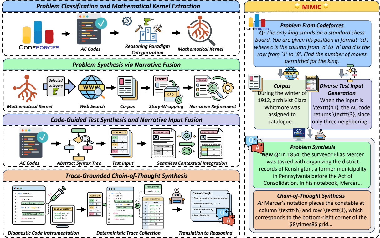
Figure 2: Overview of the MIMIC framework. It transforms raw algorithmic problems into verifiable reasoning data through a four-stage pipeline: (1) Problem Classification and Mathematical Kernel Extraction, (2) Problem Synthesis via Narrative Fusion, (3) Code-Guided Test Synthesis and Narrative Input Fusion, and (4) Trace-Grounded Chain-of-Thought (CoT) Synthesis.
