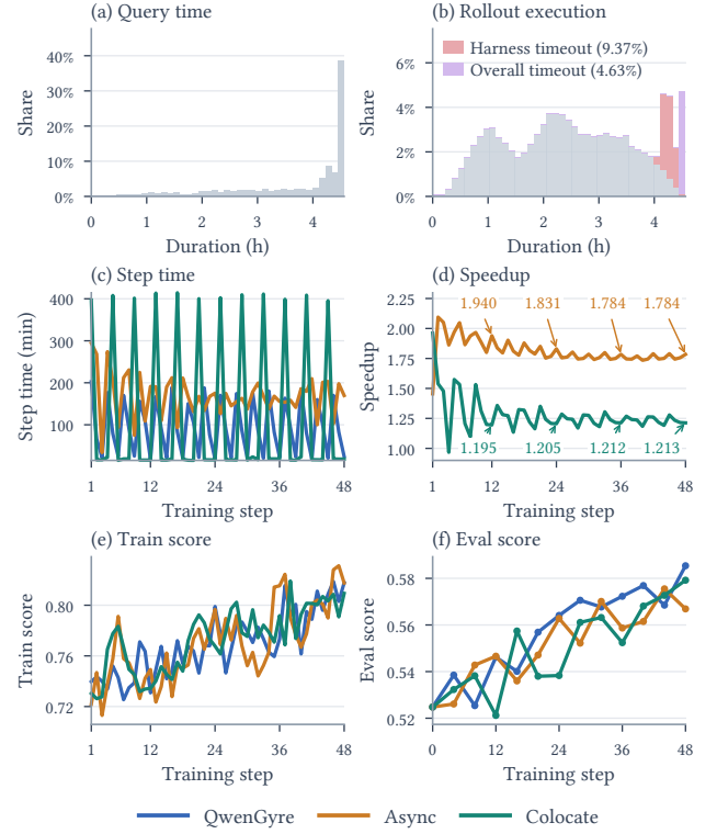
Figure 8: NL2RepoBench with Qwen 3.8 2.4T. (a) Measured query durations, using the longest rollout execution wall time per query. (b) Measured rollout execution durations. The final bin collects durations \geq 4.45 h. In (b), pink and purple mark harness and overall timeouts, respectively. (c,d) Step times and cumulative speedups over 48 steps. Arrows in (d) label speedups at selected checkpoints in matching colors. (e,f) Training and evaluation scores.
