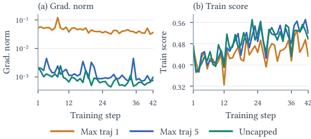
Figure 9: Trajectory-budget ablation for QWENGYRE on NL2RepoBench with Qwen 3.6 122B over training steps 1–42. (a) Gradient norm on a logarithmic scale. (b) Mean training score. Max traj 1 samples only the main trajectory per execution; Max traj 5 admits up to five trajectories; “Uncapped” uses all available leaf trajectories.
