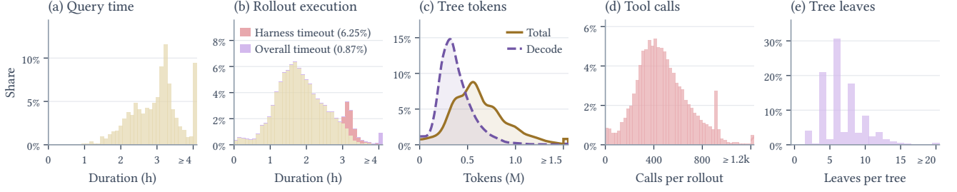
Figure 5: NL2RepoBench execution distributions with Qwen 3.6 122B at \mathbb{E}[d] = 1.5 over steps 1–48. (a) Query durations, measured as the longest of each query’s 16 rollout execution durations. (b) Rollout execution durations. (c) Total (solid) counts input and output tokens per rollout tree; Decode (dashed) counts generated output tokens. Both count shared prefixes once. The smoothed curves show shares per 50k tokens. (d) Tool calls per rollout execution. (e) Leaves per rollout tree. In (b), pink and purple mark harness and overall timeouts, respectively; executions with both flags appear only in purple. Final bins labeled \geq collect values at or above the indicated thresholds.
