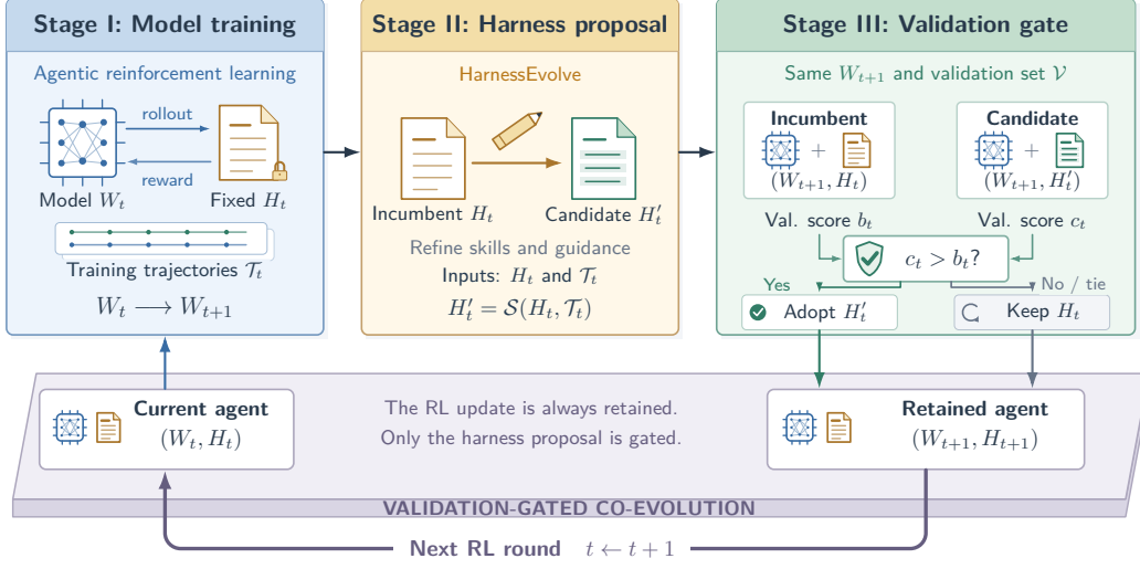
Figure 2: Overview of VACE. Stage I trains the model under the current harness and collects execution trajectories. Stage II turns this feedback into a proposed harness revision. Stage III compares the incumbent and candidate at the updated checkpoint. The retained harness then guides the next RL round, closing the feedback loop between model training and harness refinement.
