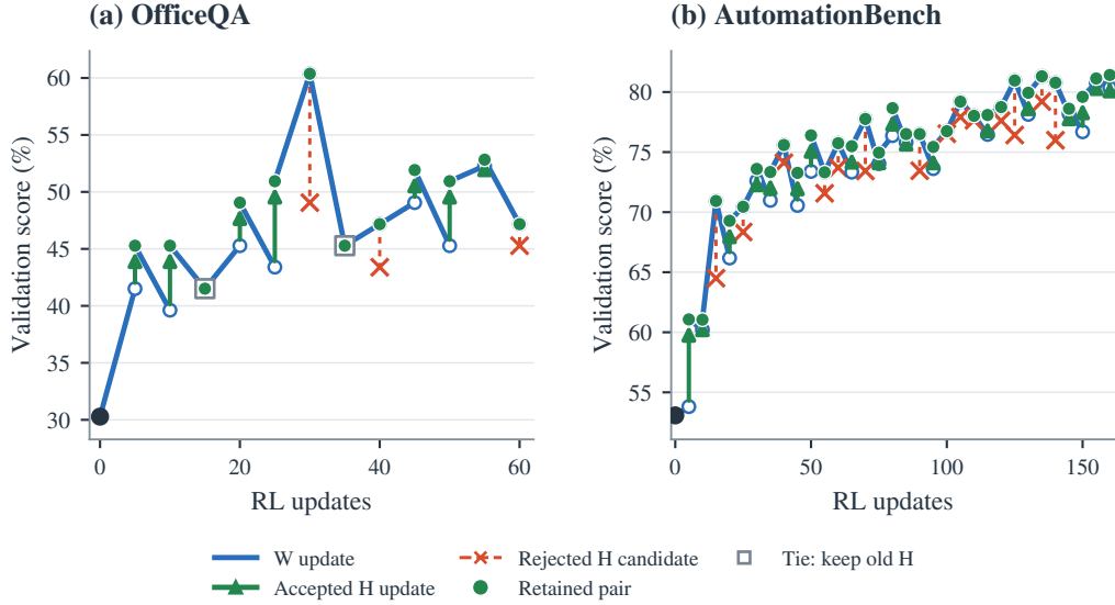
Figure 3: Phase-level validation dynamics. Blue segments connect a retained pair to the next post-weight evaluation; green arrows mark accepted harness updates, red crosses rejected candidates, and outlined squares ties. Green dots identify retained pairs, from which the next weight stage starts.
