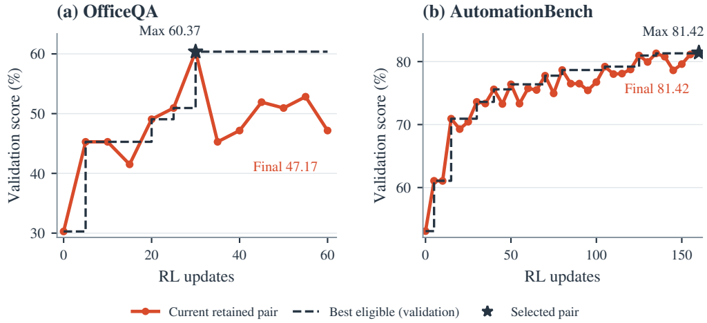
Figure 5: Validation trajectories. Solid curves show the scores after each round, dashed curves show the best scores reached so far, and stars mark the maxima.
