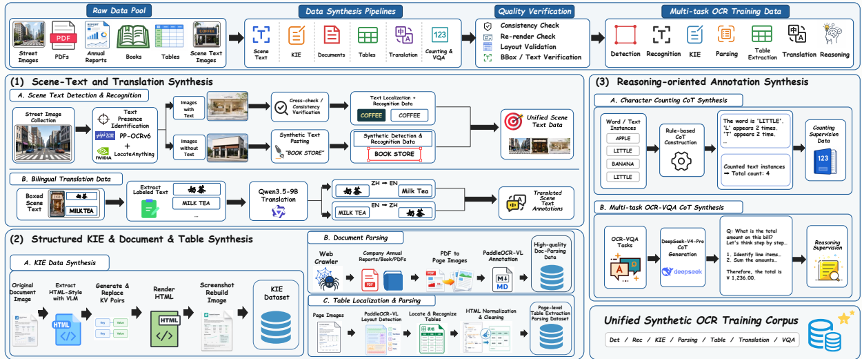
Figure 3 Overview of the targeted data-construction engine. Heterogeneous raw assets are transformed into task-specific supervision for scene-text detection and recognition, bilingual translation, key information extraction, document parsing, Chinese table localization and parsing, and OCR-centric reasoning.
