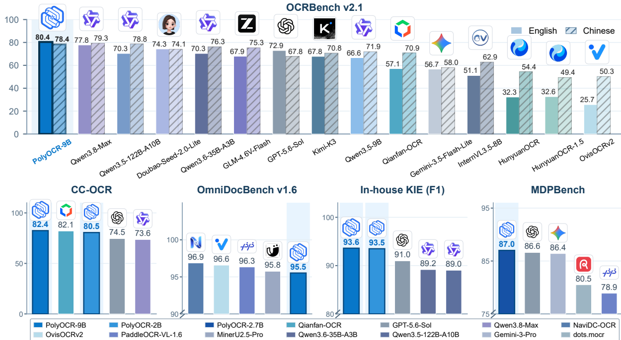
Figure 1 Cross-benchmark comparison. OCRBench v2.1 is shown above; CC-OCR, OmniDocBench v1.6, in-house KIE, and MDPBench are shown below with representative baselines. OmniDocBench uses the PolyOCR-9B layout-guided pipeline, whereas MDPBench uses PolyOCR-2.7B. CC-OCR excludes multilingual OCR; truncated axes are marked.
