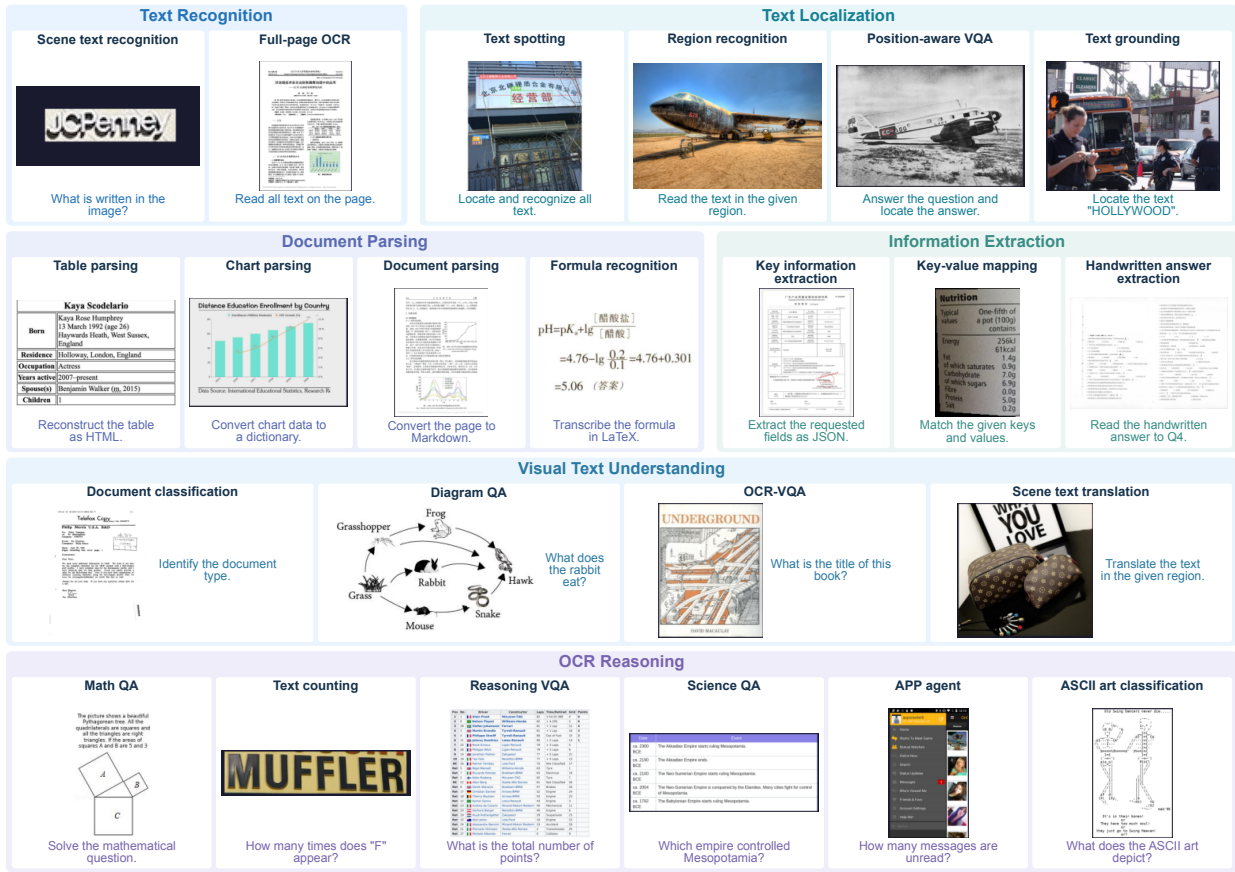
Figure 2 Representative tasks across the six OCR capability dimensions. Each card pairs an example image with a shortened instruction. The gallery combines task illustrations from Table 16 with selected examples from OCRBench v2 (Fu et al., 2025); the displayed examples illustrate task definitions rather than the composition of the training corpus.
