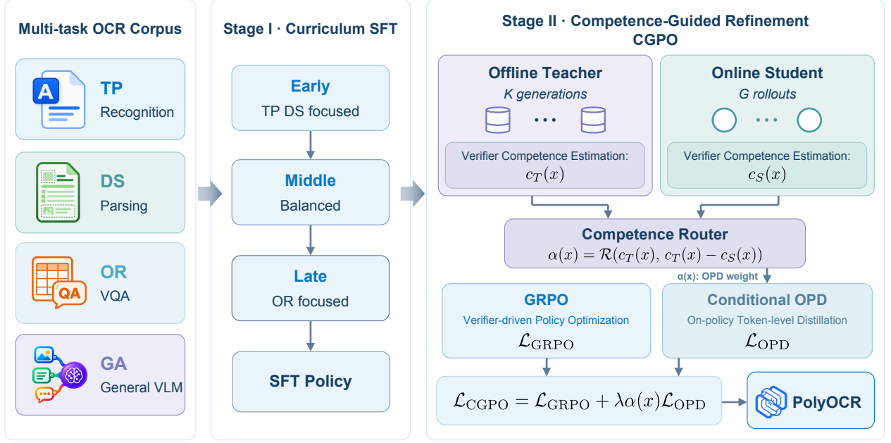
Figure 4 Overview of the PolyOCR training framework. Stage I applies a three-phase curriculum SFT schedule over Text Perception (TP), Document Structure Understanding (DS), OCR Understanding and Reasoning (OR), and General Multimodal Alignment (GA) data. Stage II performs CGPO by combining verifier-driven GRPO with conditional OPD. Here, \mathcal{R} denotes the calibrated competence-routing map defined in Sec. 4.3, which maps the cached teacher competence c_T(x) and teacher–student competence gap c_T(x) - c_S(x) to the OPD weight \alpha(x) .
