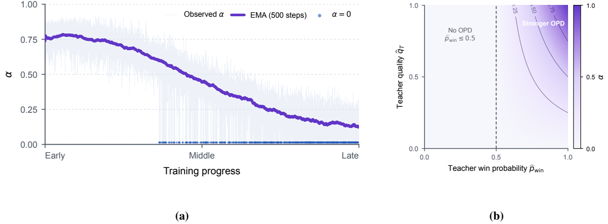
Figure 5 CGPO routing behavior. (a) Observed routing coefficients during CGPO, their exponential moving average, and points with \alpha = 0 . (b) Analytical routing surface induced by \alpha = \hat{q}_T(2\hat{p}_{win} - 1)_+ . OPD is disabled when \hat{p}_{win} \leq 0.5 and receives increasing weight as teacher quality and the calibrated probability of teacher superiority increase.
