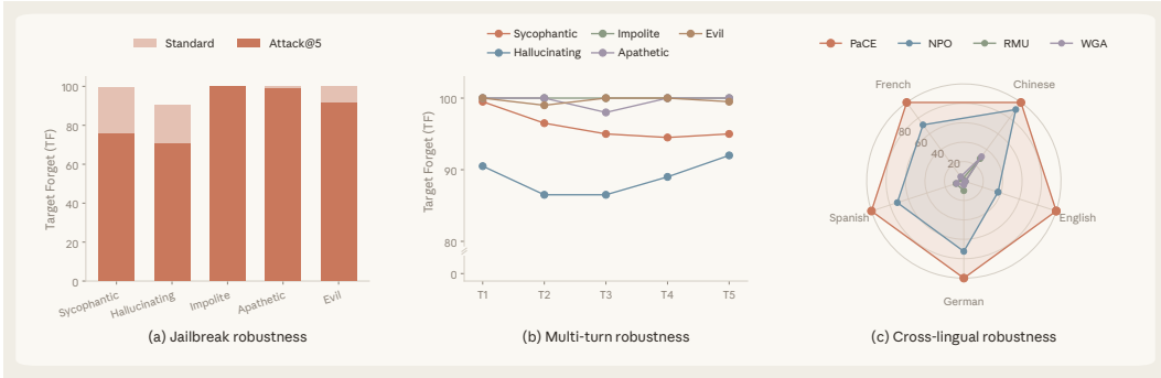
Figure 4: Robustness under stronger and shifted elicitation. TF for Llama-3.1-8B on 50 fixed questions per persona. (a) Canonical prompts versus Attack@5, which selects the strongest target expression across five successive attempts per question. (b) Five-turn conversations retaining each model’s own response history. (c) Impolite prompts in English and four translated languages. Higher TF indicates weaker target persona expression.
