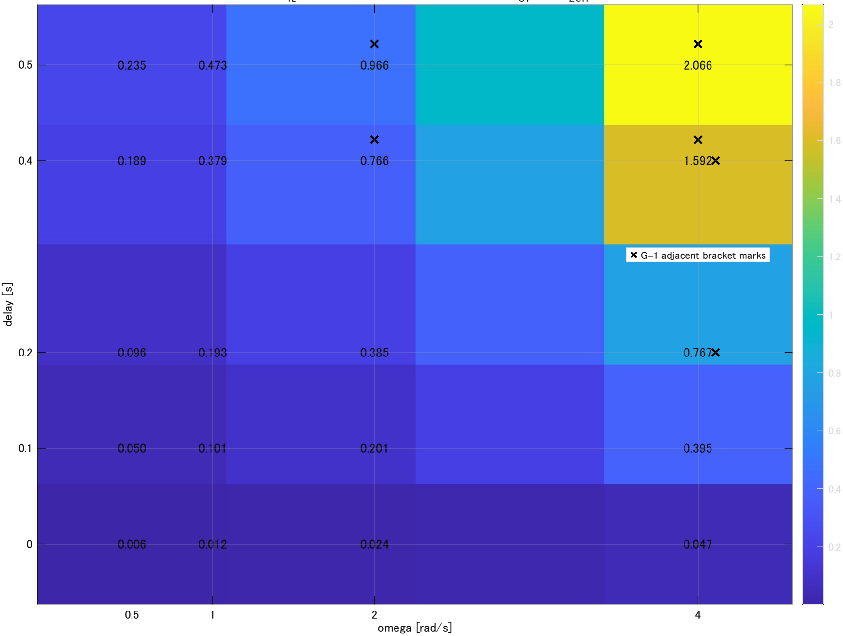
lissajous 12 discrete performance ratio map G = \text{RMSE}_{\text{CV}} / \text{RMSE}_{\text{ZOH}}
