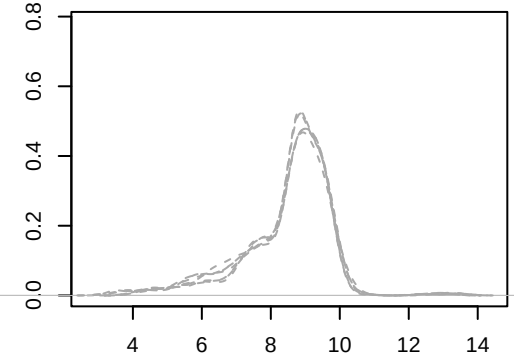
RLR
