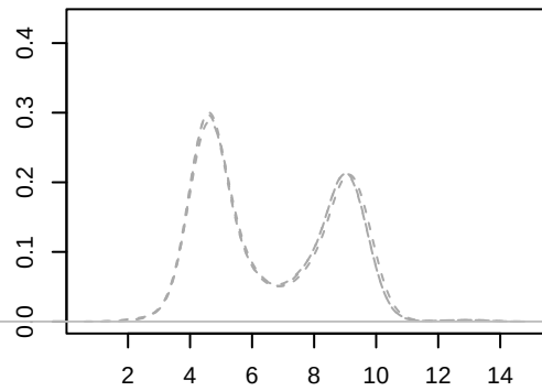
log2
