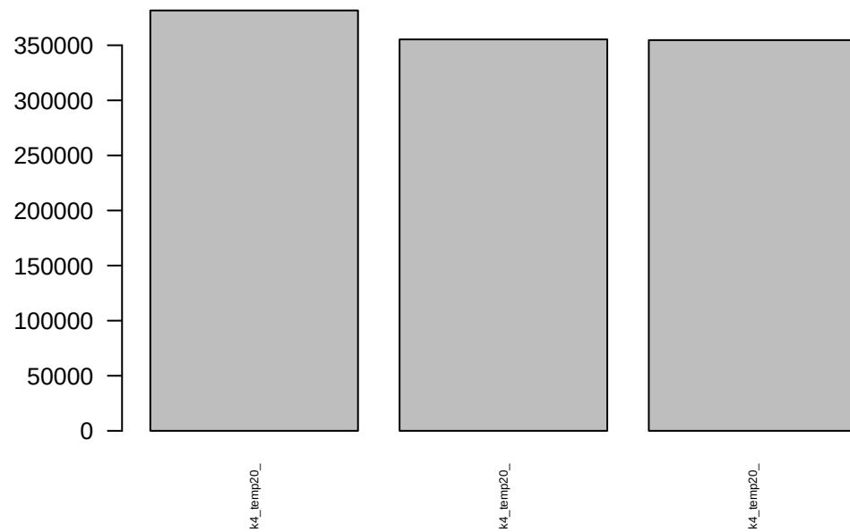
Total intensity
