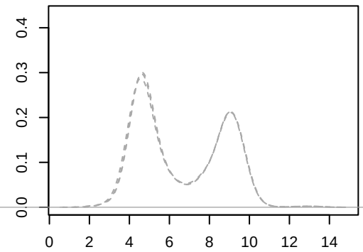
median
