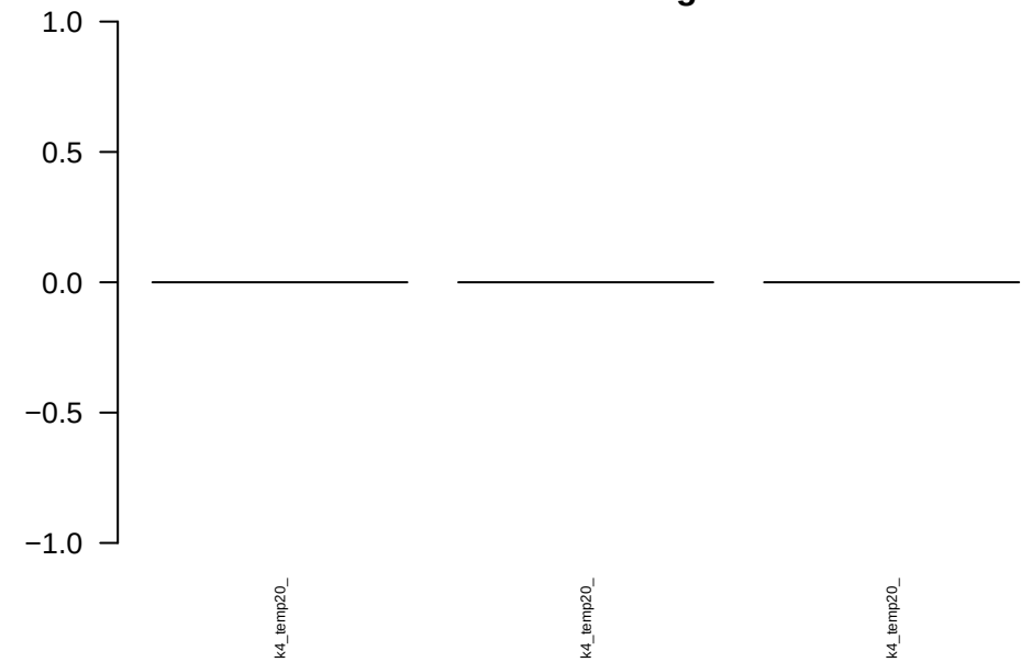
Total missing
