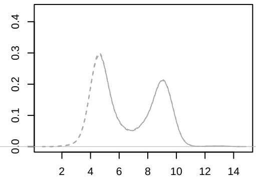
RLR
