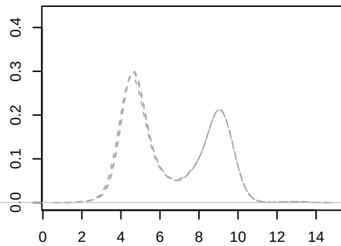
mean
