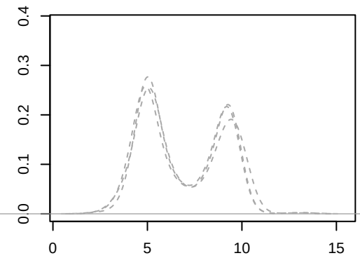
median
