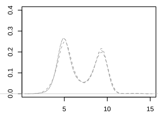
RLR
