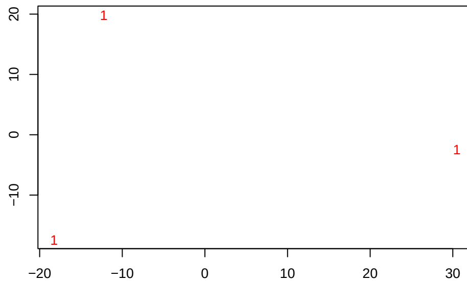
Log2-MDS plot
