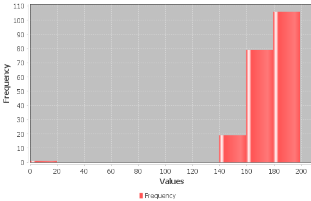
Data Distribution
