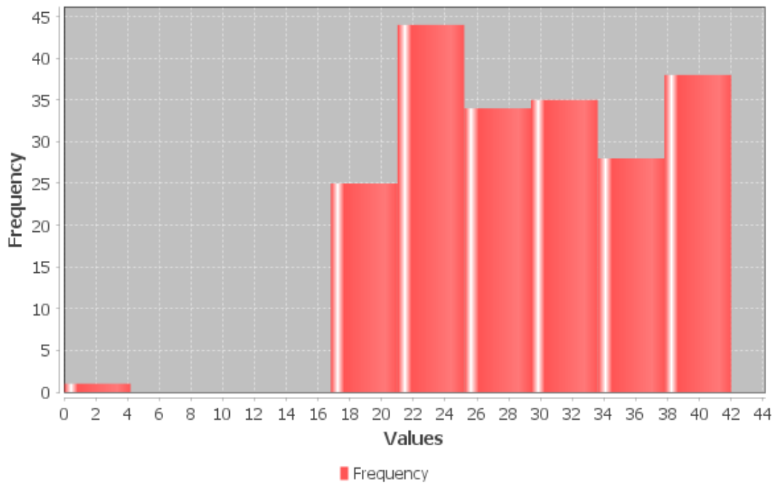
Data Distribution
