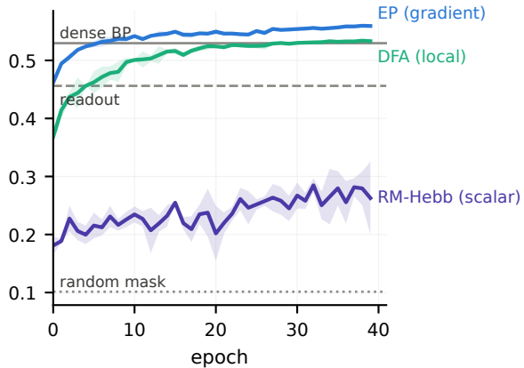
CIFAR-10
