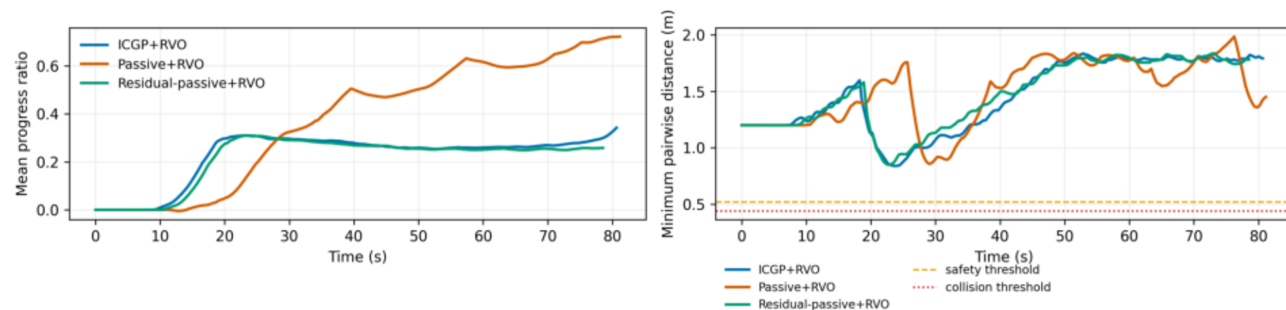
Time-resolved metrics derived from raw Gazebo CSV logs
