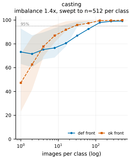
Per-class data efficiency on four industrial defect datasets (line = mean over 11 models x 5 seeds, band = interquartile range)
