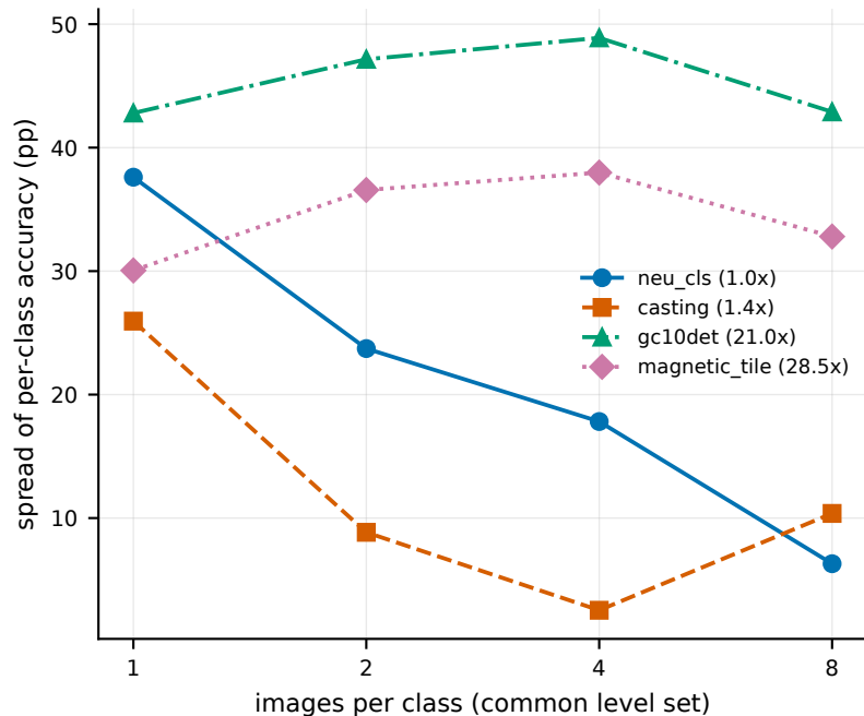
(b) At an equal budget the imbalanced sets keep a 5x larger class gap
