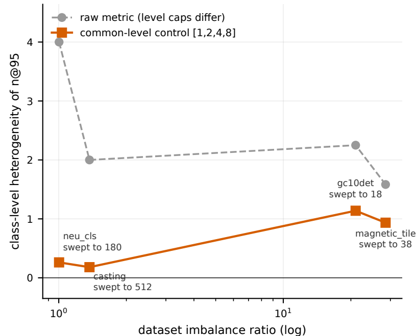
(a) Imbalance amplifies heterogeneity once the dynamic range is controlled
