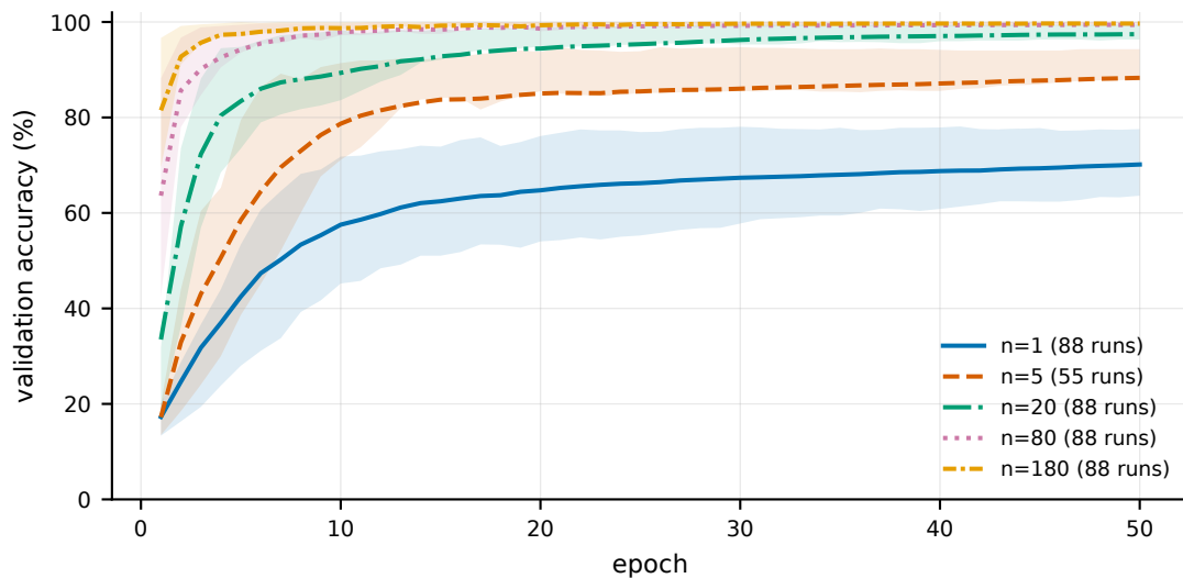
(c) Best epoch arrives earlier as data grows (median 34 -> 9 epochs as n goes 1 -> 180)
