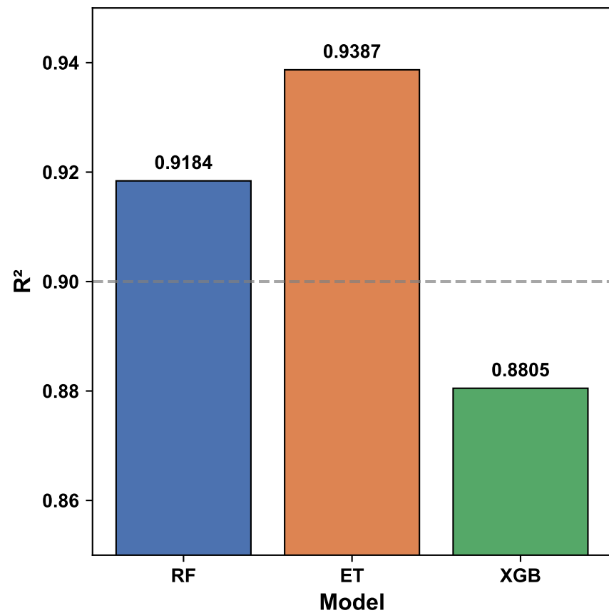
(a) R^2 Score
