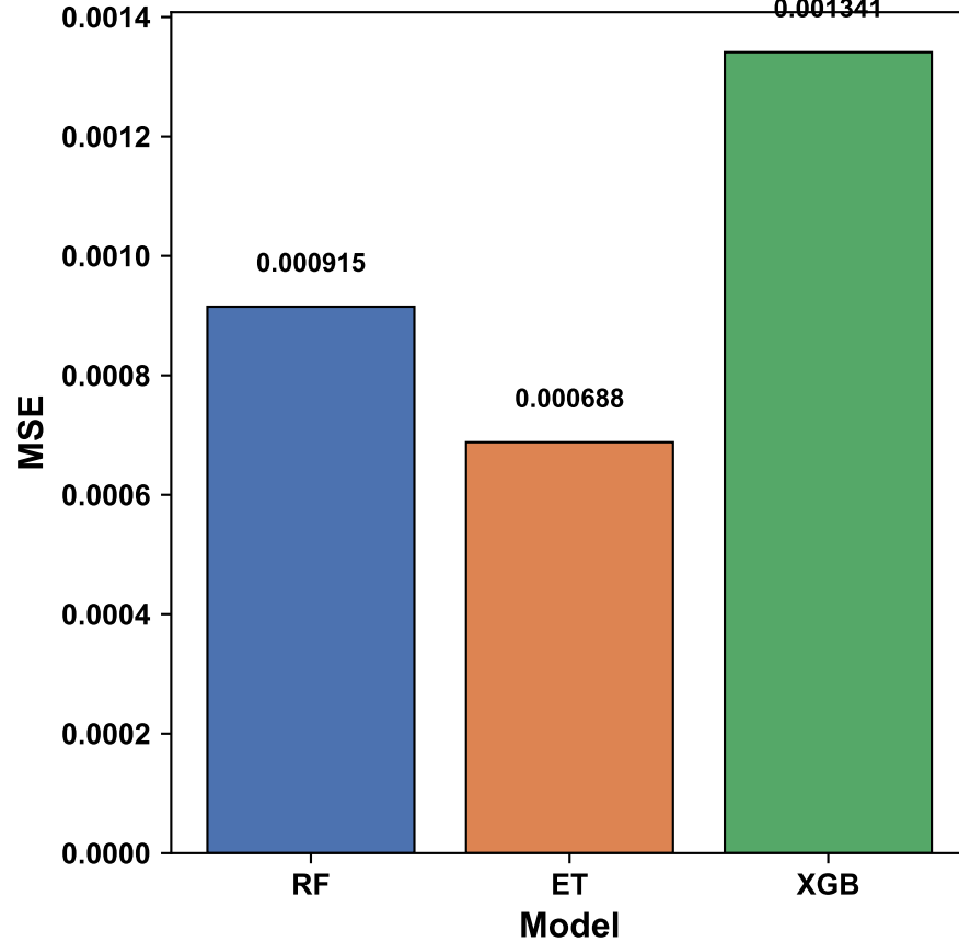
(b) Mean Squared Error
