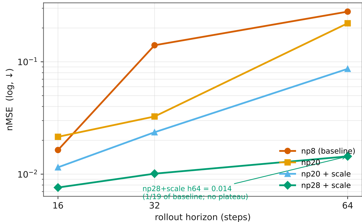
Real data (Physion++): the longer the training rollout, the better the long horizon
