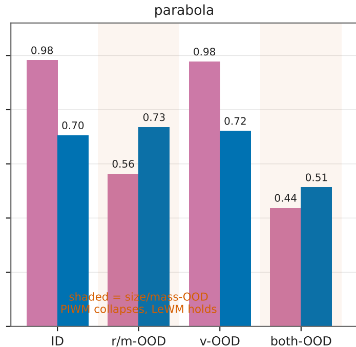
PIWM learns clean physics (wins ID & v-OOD) but its VAE encoder collapses on size/mass-OOD
