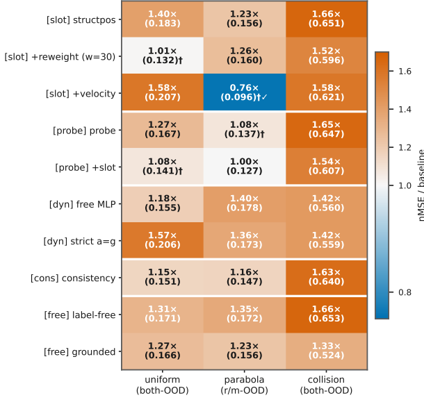
Figure 2: Every injection variant \times domain against the free-rollout baseline (nMSE ratio; \dagger = three-seed mean, others single-seed). Vermillion = worse, white = parity, blue = better. Injection is at or below baseline in 29 of 30 cells (25 worse, 4 parity); the collision column (1.33–1.66 \times ) is uniformly worst; the sole real gain is velocity+slot on parabola (0.76 \times , \dagger\checkmark ).
