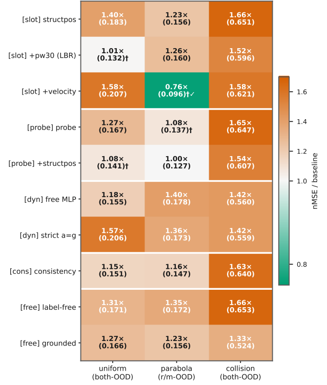
Figure 2: Every injection variant \times domain against the free-rollout baseline (nMSE ratio; number = single-seed value, \dagger = three-seed mean). Red = worse, white = parity, green = better. Injection is at or below baseline in 29 of 30 cells (25 worse, 4 parity); the collision column ( 1.33\text{--}1.66\times ) is uniformly worst; the sole real gain is velocity+slot on parabola ( 0.76\times , \dagger\checkmark ).
