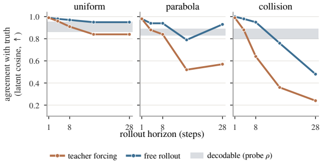
Figure 3: Decodable, yet drifting—one panel per domain. In each, the shaded band is that domain’s position decodability from frame embeddings (both- \text{OOD} probe \rho , per coordinate): high everywhere (0.80–0.96), no decay with horizon. The teacher-forced rollout (orange) falls out of the band by an amount tracking dynamics complexity (horizon-28 latent cosine: 0.84 uniform, 0.57 parabola, 0.24 collision, from 0.98–0.99 at one step); free rollout (blue) recovers much of the gap with no physics added.
