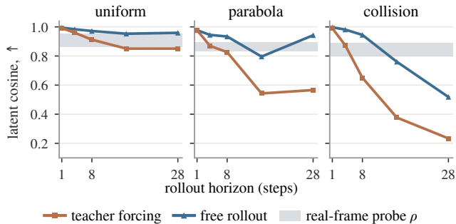
Figure 3: Decodable, yet drifting—one panel per domain. In each, the gray band is a horizon-independent reference: position decodability from real-frame embeddings (both-OOD probe \rho , one bound per coordinate), high everywhere (0.80–0.96). Curves show three-seed mean latent cosine. The teacher-forced rollout (orange) falls away by an amount tracking dynamics complexity (horizon-28 cosine: 0.85 uniform, 0.57 parabola, 0.23 collision, from 0.98–0.99 at one step); free rollout (blue) recovers much of the gap with no physics added.
