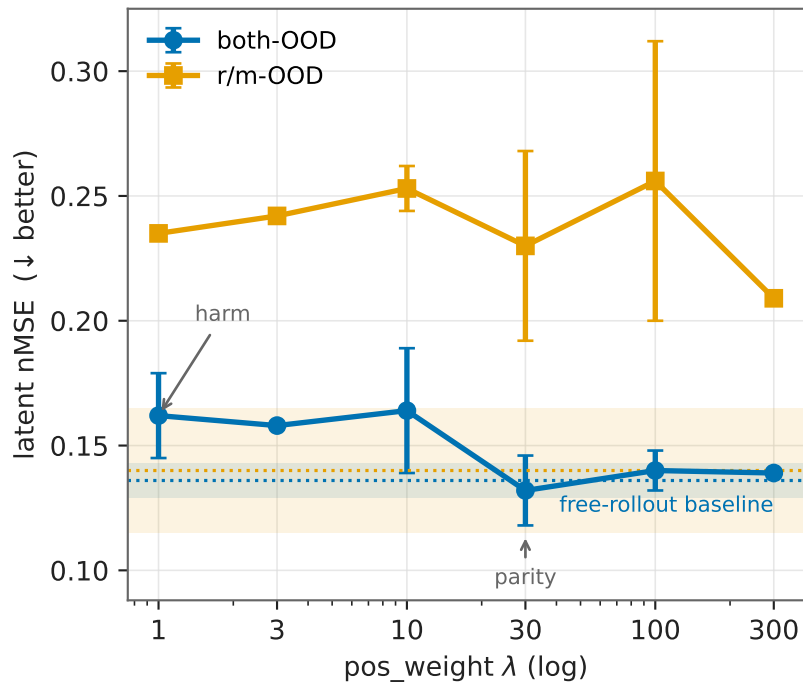
(a) uniform: both-OOD \rightarrow parity, r/m-OOD never
