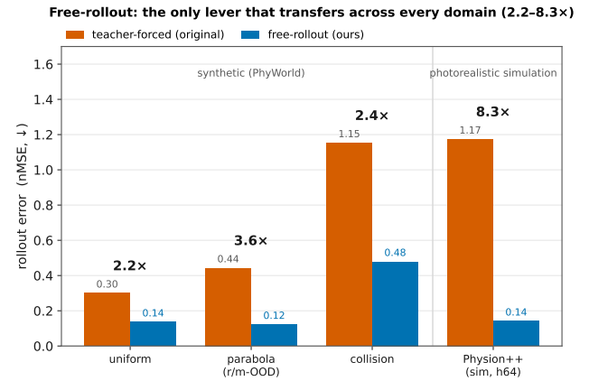
Figure 5: Teacher forcing vs. free rollout (hardest clean split, nMSE \downarrow ; fold-change above bars). One training-protocol switch, injecting no physics: uniform 0.300 \rightarrow 0.136 (2.2 \times ), parabola 0.443 \rightarrow 0.122 (3.6 \times ), collision 1.153 \rightarrow 0.479 (2.4 \times ), Physion++ horizon-64 1.174 \rightarrow 0.141 (8.3 \times ); all three-seed with non-overlapping intervals.
