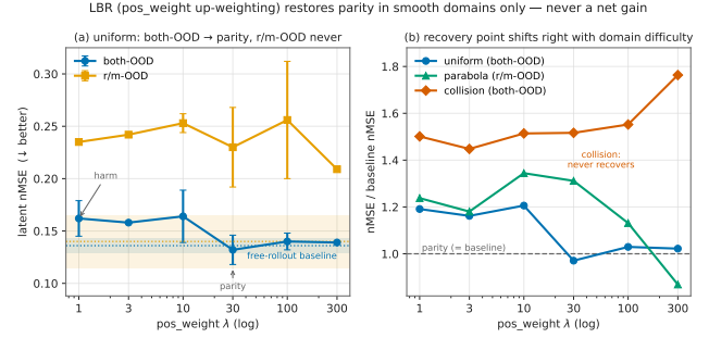
Figure 4: Dose–response re-weighting. Left: uniform, slot weight 1 \rightarrow 300 against the baseline band—both-OOD returns to parity, r/m -OOD never does. Right: nMSE ratio to baseline across domains—collision stays above baseline at every weight and degrades as weight grows. Re-weighting validates the mechanism’s direction but is not a repair.
