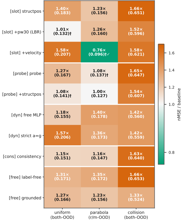
Figure 2: Every injection arm \times domain against the free-rollout baseline (nMSE ratio; number = single-seed value, \dagger = three-seed mean). Red = worse, white = parity, green = better. Injection is at or below baseline in 29 of 30 cells (25 worse, 4 parity); the collision column (1.33–1.66 \times ) is uniformly worst; the sole real gain is velocity+slot on parabola (0.76 \times , \dagger\checkmark ).
