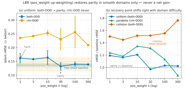
Figure 4: Dose-response re-weighting. Left: uniform, slot weight 1 \rightarrow 300 against the baseline band—both-ODD returns to parity, r/m-ODD never does. Right: nMSE ratio to baseline across domains—collision stays above baseline at every weight and degrades as weight grows. Re-weighting validates the mechanism’s direction but is not a repair.
