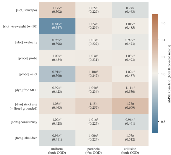
Figure 6: The injection scan repeated on the frozen-DINOv2 backbone, drawn and judged exactly as Figure 2 (three-seed means over three-seed baseline; o = the cell’s seeds overlap the baseline’s; the a=g /grounded row merged, four draws). 3 cells worse in every seed / 23 within noise / 1 below (26 of 27 fail to improve on baseline; the one cell below 1.0 separates by only a 0.001 margin at 0.97 \times ). The dynamics-head row is the worst here too (1.27 \times on collision); the visually blue uniform cells are all within noise and additionally dissolve under the content-free controls of Trap 5.
