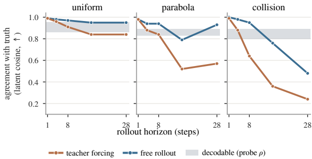
Figure 3: Decodable, yet drifting—one panel per domain. In each, the shaded band is that domain’s position decodability from frame embeddings (both-OOD probe \rho , per coordinate): high everywhere (0.80–0.96), no decay with horizon. The teacher-forced rollout (orange) falls out of the band by an amount tracking dynamics complexity (horizon-28 latent cosine: 0.84 uniform, 0.57 parabola, 0.24 collision, from 0.98–0.99 at one step); free rollout (blue) recovers much of the gap with no physics added.
