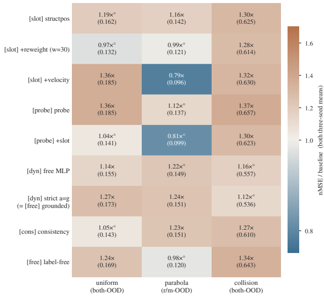
Figure 2: Every injection variant \times domain vs. the free-rollout baseline (nMSE ratio; every cell and the baseline are three-seed means). Warm = worse, blue = better; ^{\circ} = within noise (the cell’s seeds overlap the baseline’s). Injection fails to improve on baseline in 26 of 27 cells (15 worse, 11 within noise); the sole seed-robust gain is velocity+slot on parabola (0.79 \times ). Strict a=g and the grounded prior are one configuration launched twice; the merged row pools all four draws.
