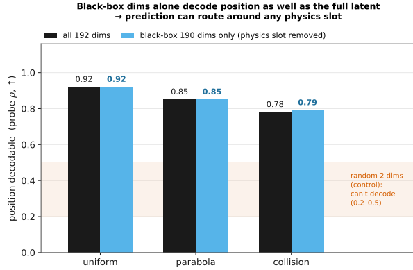
Figure 3: Direct evidence of the bypass. Per domain: position decoded from all 192 dimensions (dark) vs. from the 190 black-box dimensions alone (blue) are nearly equal (0.78–0.92); a random 2-dimension control (band) fails. The black box redundantly encodes position, so prediction need not consult an injected slot.
