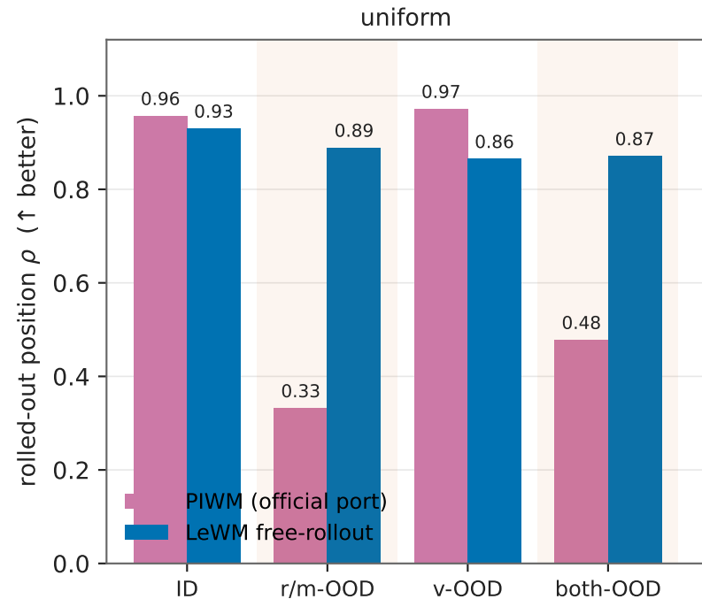
PIWM learns clean physics (wins ID & v-OD) but its VAE encoder collapses on size/mass-OD
