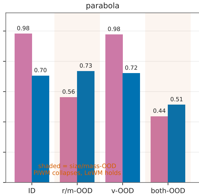
PIWM learns clean physics (wins ID & v-OD) but its VAE encoder collapses on size/mass-OD
