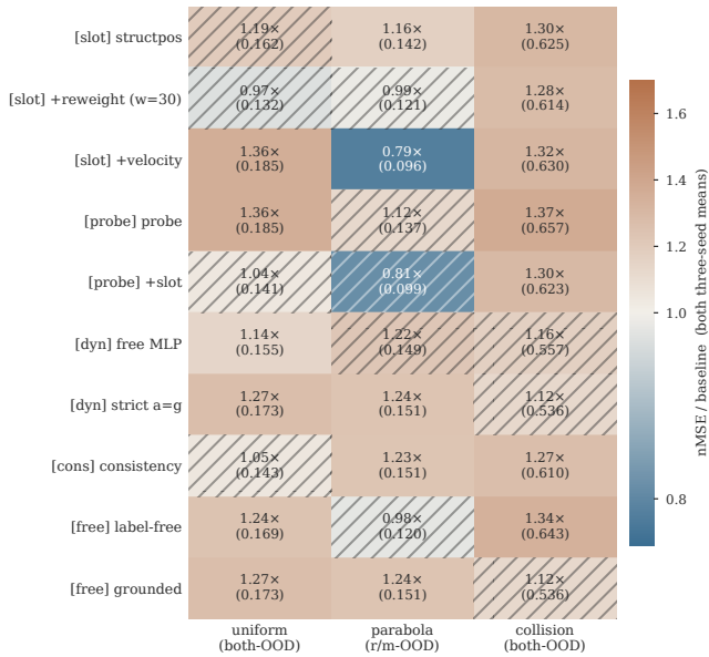
Figure 2: Every injection variant \times domain vs. the free-rollout baseline (nMSE ratio; every cell and the baseline are three-seed means). Warm = worse, blue = better; hatched = within noise (the cell’s seeds overlap the baseline’s), solid = separated in every seed. Injection is at or below baseline in 29 of 30 cells (17 worse, 12 within noise); the sole seed-robust gain is velocity+slot on parabola (0.79 \times ). The a=g and grounded rows are the same configuration (see text).
