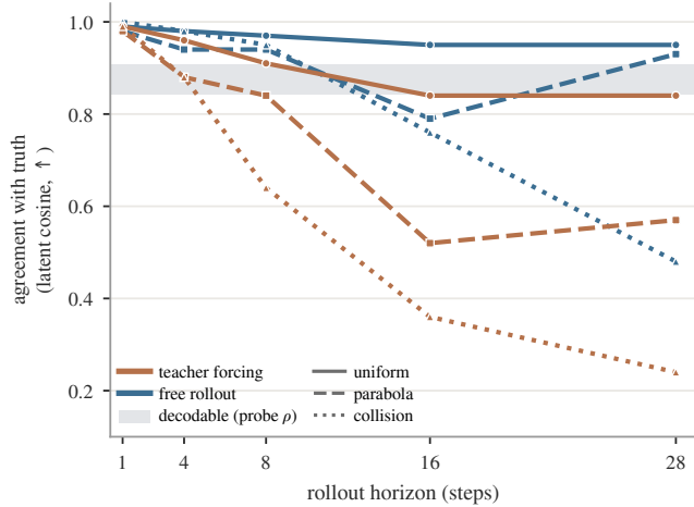
Figure 3: Decodable, used, and still drifting. The shaded band is position decodability from frame embeddings (both-OOD probe \rho ): present everywhere (0.84–0.91), no decay with horizon. The teacher-forced rollout falls out of the band by an amount tracking dynamics complexity (horizon-28: 0.84 uniform, 0.57 parabola, 0.24 collision, from 0.98–0.99 at one step); free rollout recovers much of the gap with no physics added.
