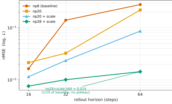
Physion++ (photorealistic simulation): longer training rollout → better long horizon
