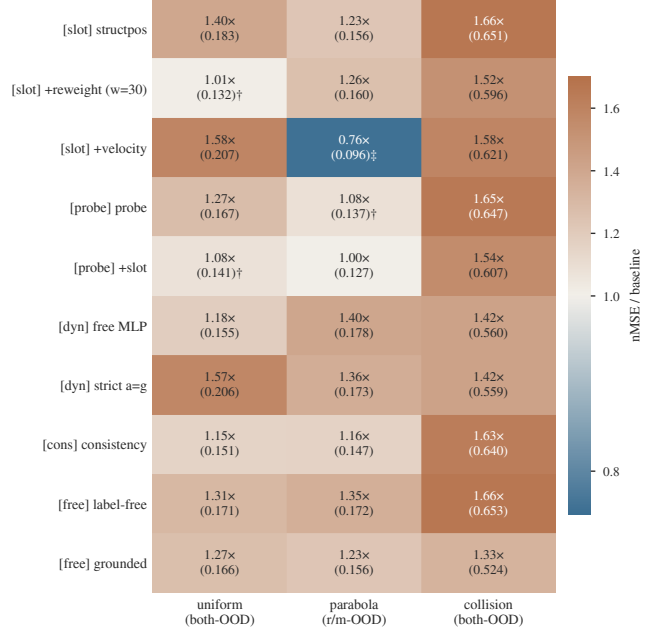
Figure 2: Every injection variant \times domain against the free-rollout baseline (nMSE ratio; † = three-seed mean and ‡ = three-seed mean that beats baseline, others single-seed). Warm = worse, pale = parity, blue = better. Rows follow the three groups of Table 1 in order, and each row label prefixes its mechanism. Injection is at or below baseline in 29 of 30 cells (25 worse, 4 parity); the collision column ( 1.33\text{--}1.66\times ) is uniformly worst; the sole real gain is velocity+slot on parabola ( 0.76\times , ‡).
