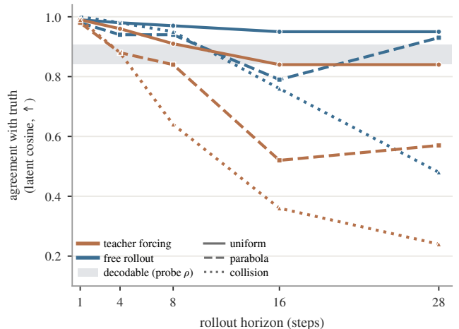
Figure 3: Decodable, but not load-bearing, in all three domains. Colour is the training protocol; line style is the domain. The shaded band is position decodability from the frame embeddings (both-OOD probe \rho , mean over both coordinates): the state is present to the same degree everywhere (0.84–0.91) and does not decay with horizon. The teacher-forced rollout nevertheless falls out of that band by an amount that tracks dynamics complexity—at horizon 28 it reaches 0.84 on uniform motion, 0.57 on parabola and 0.24 on collision, from 0.98–0.99 at one step. Free rollout (§3.4) recovers much of the gap with no physics added.
