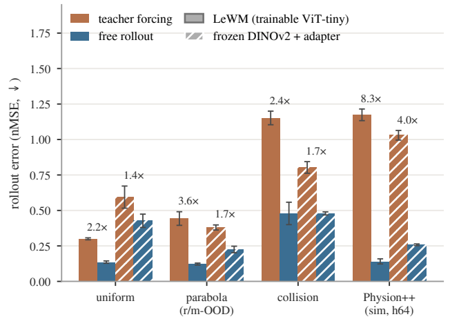
Figure 4: Teacher forcing vs. free rollout, both backbones on one axis (hardest clean split, nMSE ↓; solid = LeWM, hatched = the frozen-DINOv2 variant of §3.5; fold-change above each pair). Bars are three-seed means, error bars one sample std over seeds 3072/1234/42: every teacher-forcing/free-rollout interval is disjoint. The physics-free protocol switch is worth 2.2–8.3 \times on LeWM and 1.4–4.0 \times on frozen DINOv2—the lever is backbone-independent, and largest where the dynamics are hardest (collision, Physion++).
