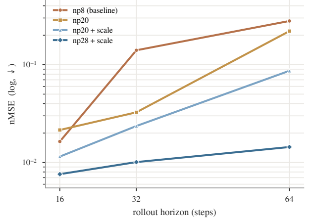
Figure 7: Physion++ direct training: per-horizon rollout nMSE (log scale) as the training horizon grows ( H=8\rightarrow 28 , +scale jitter). Long-horizon error falls monotonically to 1/19 of baseline with no inflection: realistic-simulation dynamics reward long-rollout training more than the synthetic domains do.
