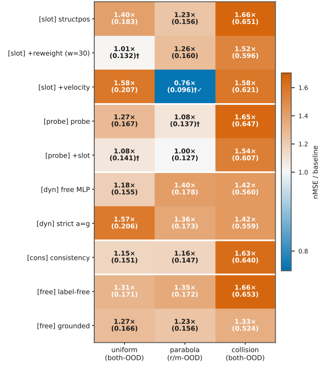
Figure 2: Every injection variant \times domain against the free-rollout baseline (nMSE ratio; † = three-seed mean, others single-seed). Vermillion = worse, white = parity, blue = better. Injection is at or below baseline in 29 of 30 cells (25 worse, 4 parity); the collision column ( 1.33\text{--}1.66\times ) is uniformly worst; the sole real gain is velocity+slot on parabola ( 0.76\times , †✓).
