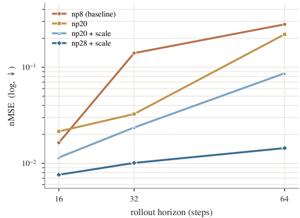
Figure 7: Physion++ direct training: per-horizon rollout nMSE (log scale) as the training horizon grows ( H=8 \rightarrow 28 , +scale jitter). Long-horizon error falls monotonically to 1/19 of baseline with no inflection: realistic-simulation dynamics reward long-rollout training more than the synthetic domains do.
