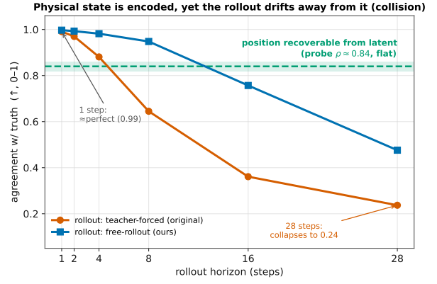
Figure 3: Decodable, but not load-bearing (collision domain). The flat dashed line is position decodability from the frame embeddings (probe \rho \approx 0.84 ): the state is present at every horizon. Yet the teacher-forced rollout (LeWM’s default) collapses from near-perfect one-step agreement (0.99) to 0.24 by horizon 28; training the same model by free rollout (§3.4) stabilizes the long horizon (0.48) with no physics added. Presence of the state does not imply its use by prediction.
