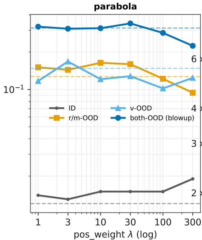
pos_weight re-weighting — absolute nMSE per partition (solid) vs its baseline (dashed, same color)
