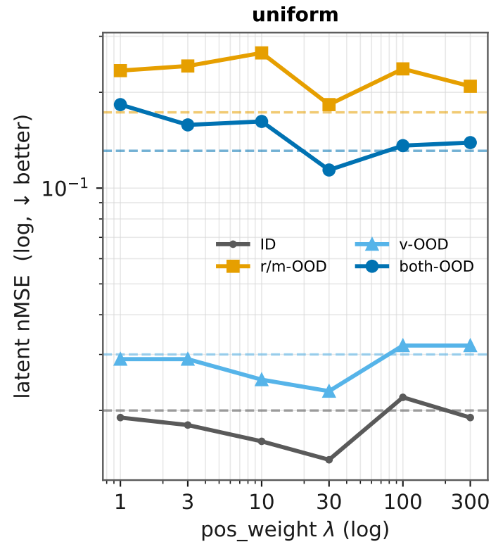
pos_weight re-weighting — absolute nMSE per partition (solid) vs its baseline (dashed, same color)
