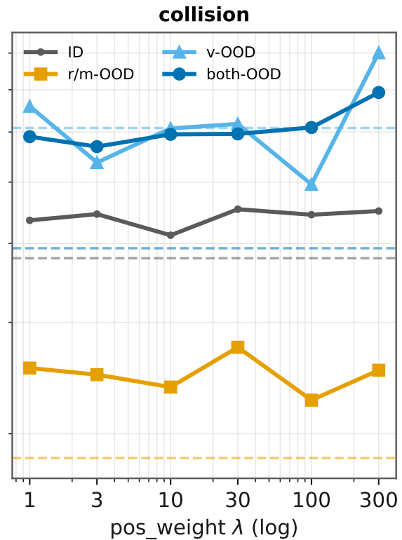
pos_weight re-weighting — absolute nMSE per partition (solid) vs its baseline (dashed, same color)
