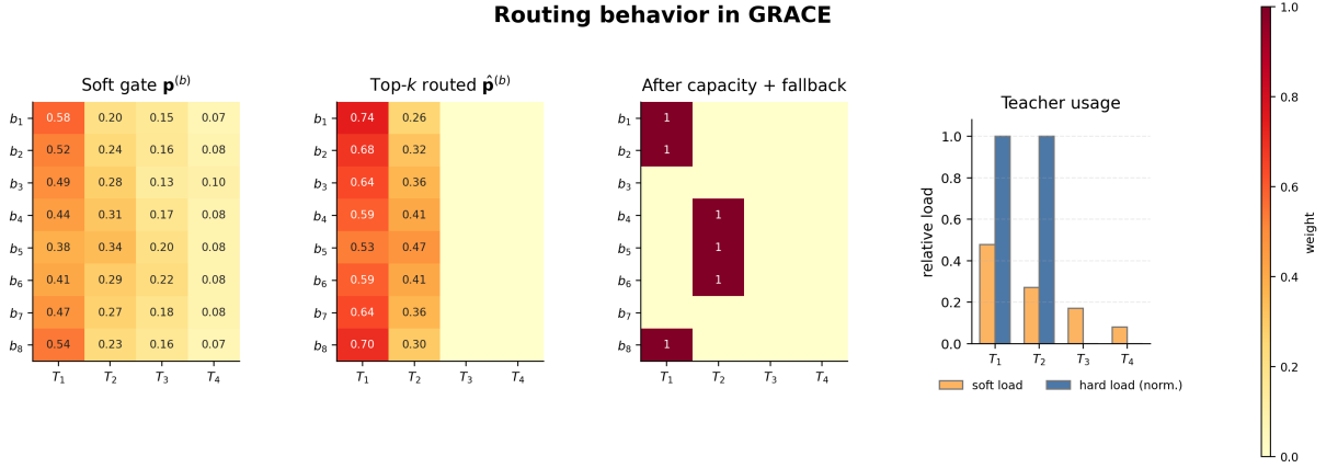
Figure 3.5: Routing dynamics in GRACE. Left to right: dense gate scores, top- k routed weights and the final assignment pattern after capacity control and fallback. The rightmost panel compares average soft load and normalized hard load, illustrating why balancing terms and expert-bias updates are needed.
