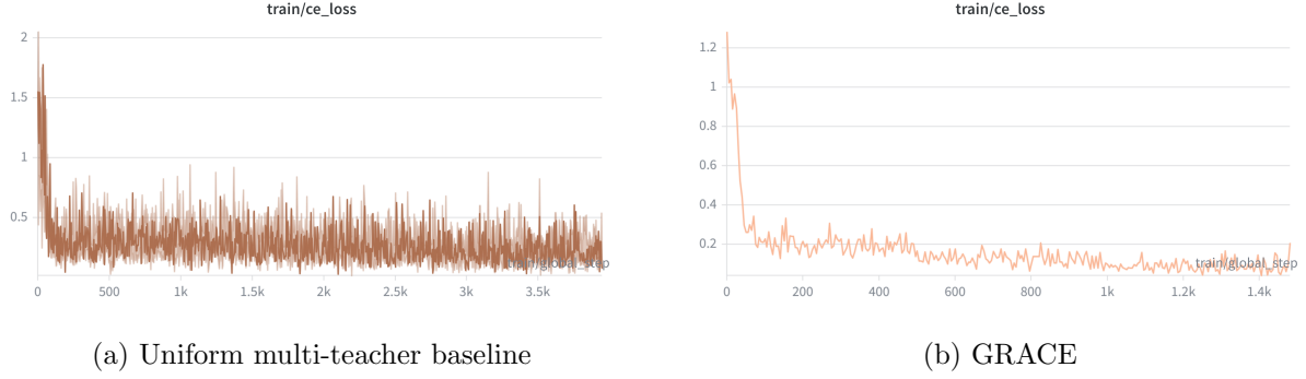
Figure 5.1: Representative training curves for the uniform multi-teacher baseline and GRACE. The GRACE curve is smoother and shows smaller oscillations, which is consistent with the claim that routing plus GRACE score refinement makes optimization more stable than static averaging.
