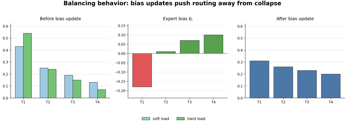
Figure 3.4: Bias-feedback behavior in GRACE under expert-bias updates. If one teacher receives too many assignments, its bias is reduced, while underused teachers receive higher bias. This shifts future routing toward a more balanced load.
