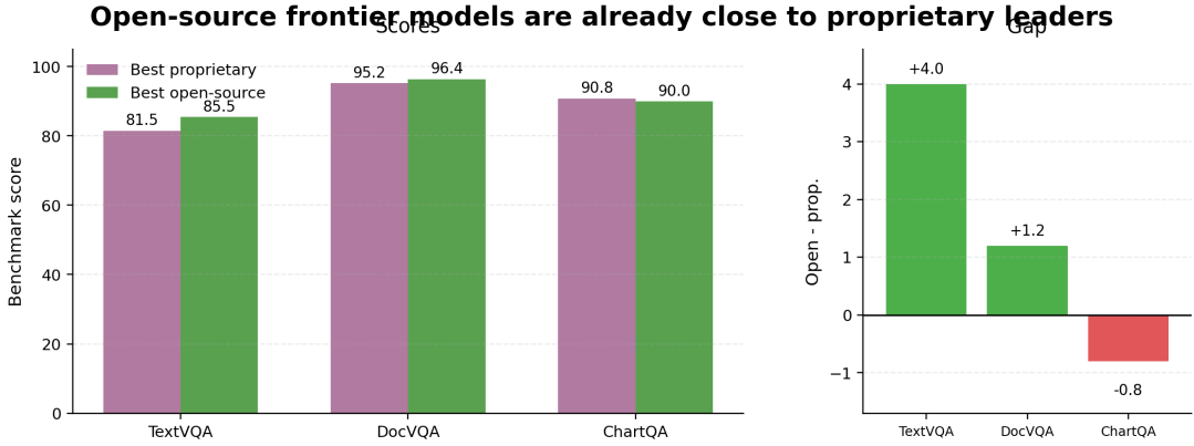
Figure 1.6: Representative proprietary and open-source frontier results on TextVQA, DocVQA and ChartQA. The gap is already small and the best open-source model is ahead on TextVQA and DocVQA. The right panel shows the benchmark gap computed as open-source score minus proprietary score from snapshots accessed on April 2, 2026 [25–27].
