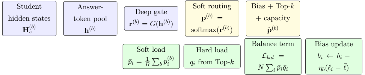
Figure 3.3: Student-conditioned routing in GRACE. Pooled student features are transformed into gate logits, converted into routing weights and sparsified by top- k and capacity constraints. The full framework includes a balance term and expert-bias updates.
