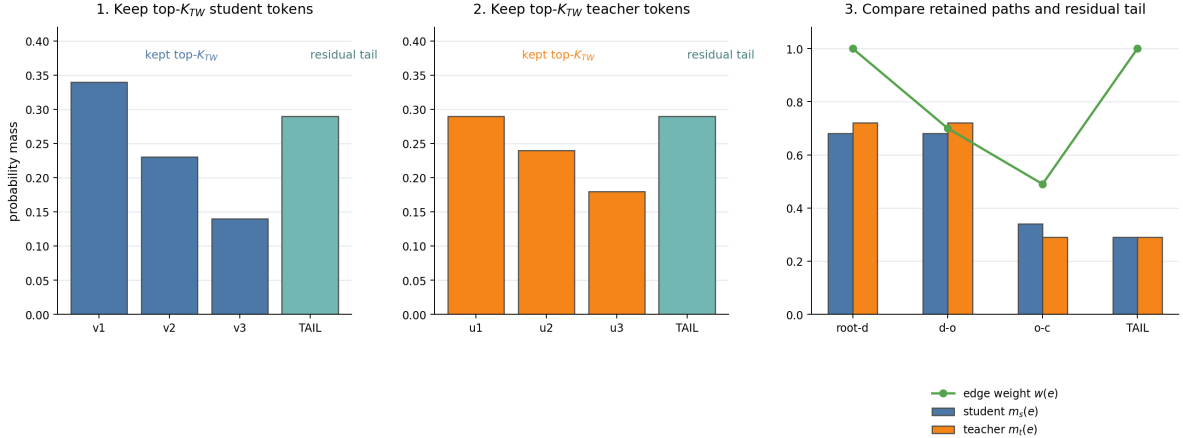
Figure 3.3: Sparse trie-Wasserstein support.
