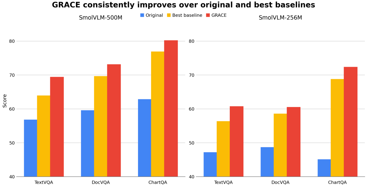
Figure 5.1: Grouped benchmark comparison.
