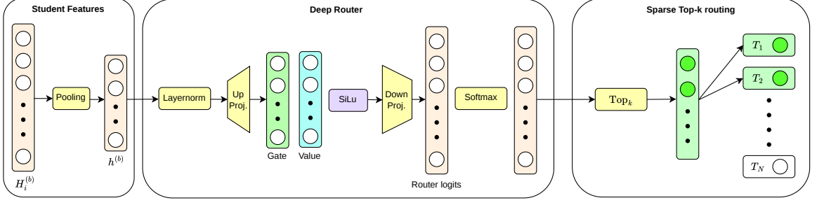
Figure 3.4: Teacher routing network.
